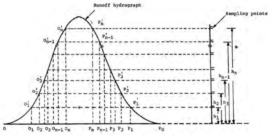
Figure 5. Working principle of the sediment sampler
