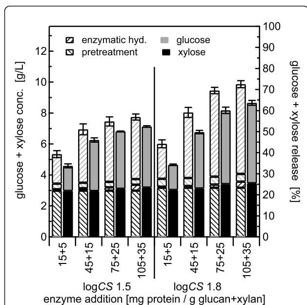
Figure 6 Dilute acid pretreatment using 1% w/w sulfuric acid with 2.0% w/w solids concentration. Glucose and xylose yields from co-hydrolysis compared with those from separate pretreatment and enzymatic hydrolysis (SPEH) for pretreatment of 2% w/w Populus slurries in 1% w/w sulfuric acid at 140°C followed by enzymatic hydrolysis over a range of enzyme loadings from 15 + 5 to 105 + 35 mg of cellulase plus xylanase, respectively, per gram of glucan and xylan in the raw biomass. The eight stacked bars on the left show pretreatment for log CS of 1.5 and those on the right for log CS of 1.8. The representation format is the same as that described in Figure 2. The error bars represent the standard errors, based three replicates.
