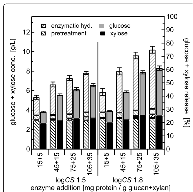
Figure 7 Dilute acid pretreatment using 2% w/w sulfuric acid with 2.0% w/w solids concentration. Glucose and xylose yields for co-hydrolysis compared with separate pretreatment and enzymatic hydrolysis (SPEH) for pretreatment of 2% w/w Populus slurries in 2% w/w sulfuric acid at 140°C followed by enzymatic hydrolysis over a range of enzyme loadings according to the same format as in Figure 6. The error bars represent the standard errors, based on three replicates.
