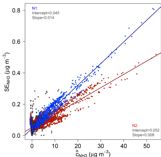
Figure 6. SE_{NH_3} vs. \hat{C}_{NH_3} (instruments N1 and N2); coloured circles represent 1 min averages, and grey circles display the difference in concentration determined by instrument N1 and N2 for half-hourly means ( \Delta_{30} = |N1 - N2| ) of the individual 1 min values; regression was carried out with the Deming method (Linnet, 1990).
