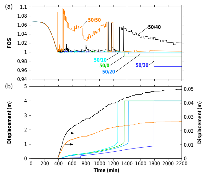
Figure 13. Time series of (a) factor of safety (FOS) and (b) displacement at the center of the slope ( x = 0 , y = 0 ) for six simulations with different tree sizes inside the clearing. The sets of two numbers shown in panel (a) indicate the stand DBH and the clearing DBH in centimeters. For example, 50/10 means a stand of trees 50 cm in diameter with a clearing filled with trees 10 cm in diameter. Spacing is identical in the clearing and in the stand (3 m). Color code is identical in panels (a) and (b). In panel (b) the simulations 50/40 and 50/50 do not fail and slope displacement plots on the vertical axis on the right side (indicated by arrows).
