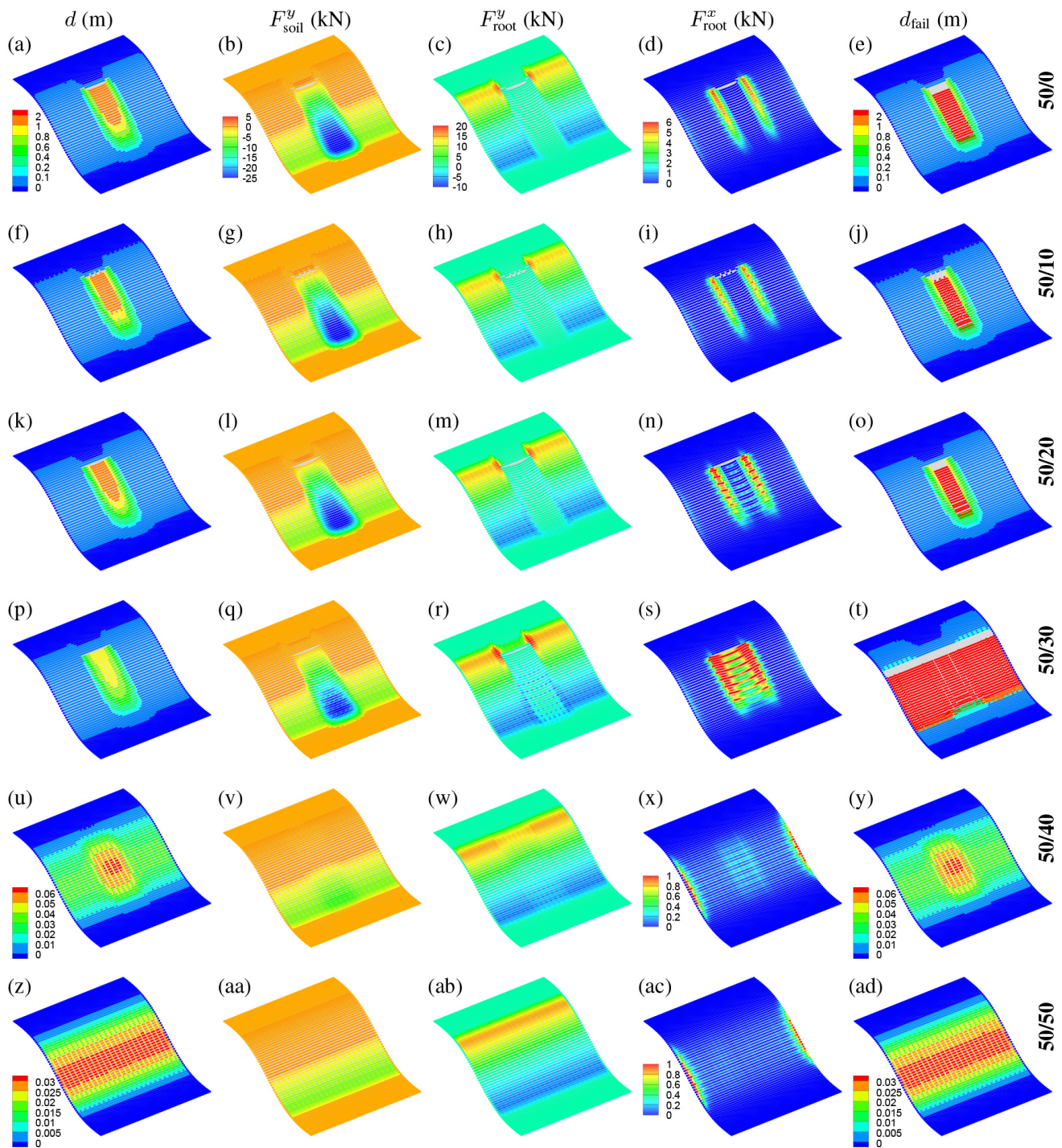
Figure 14. Effect of clearing tree size diameter on slope displacement and soil and root bond forces. From left to right, slope displacement ( d ), soil downslope compression ( F_{\text{soil}}^y ), downslope root force ( F_{\text{root}}^y ), and across-slope root force ( F_{\text{root}}^x ), at the time step just before failure and displacement at failure ( d_{\text{fail}} ) for the six simulations with different tree size diameters inside the clearing shown in Fig. 13. (a–e) Empty clearing (50/0), (f–j) DBH = 10 cm (50/10), (k–o) DBH = 20 cm (50/20), (p–t) DBH = 30 cm (50/30), (u–y) DBH = 40 cm (50/40), and (z–ad) DBH = 50 cm (50/50). Outside the clearing, DBH = 50 cm. All trees are spaced 3 m apart. Scale is given in the first row except when noted.
