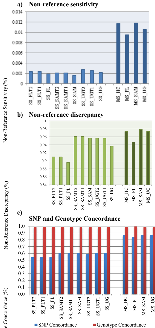
Figure 1. Single and Multi-sample caller concordance
