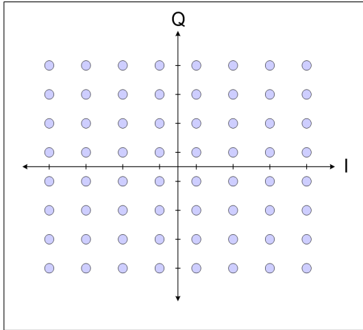
(a) 64-QAM
