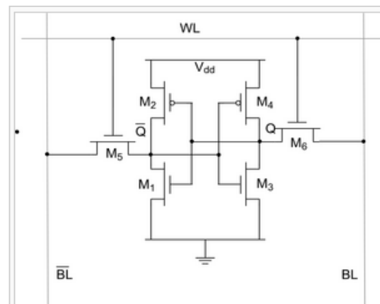
Figure 1: Basic Six-transistor SRAM cell. Two cross-coupled inverters keep the data stored as long as power is applied to the cell [22]. In the text, BL' is used to represent \overline{BL} .
