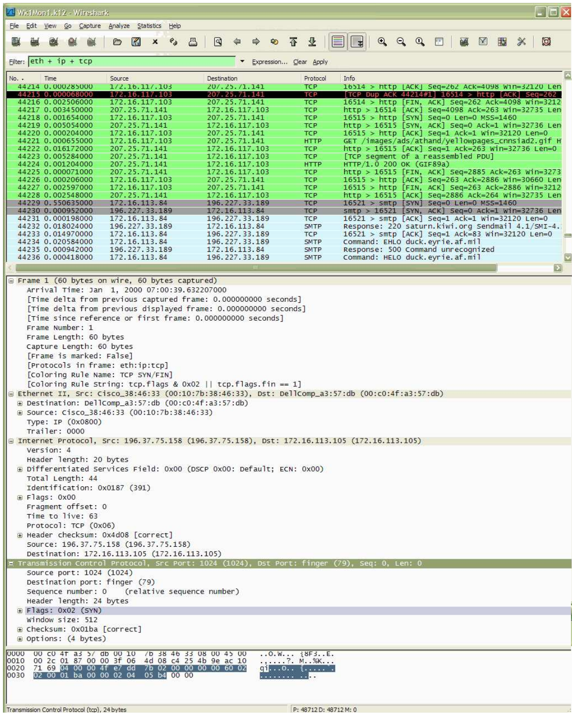
Figure 3.5: Wireshark Analyzing TCPdump File
