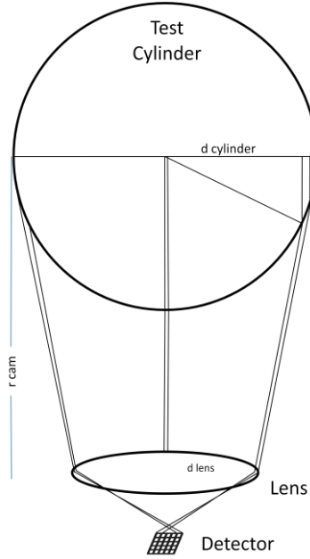
Figure 19. Geometric Alignment
