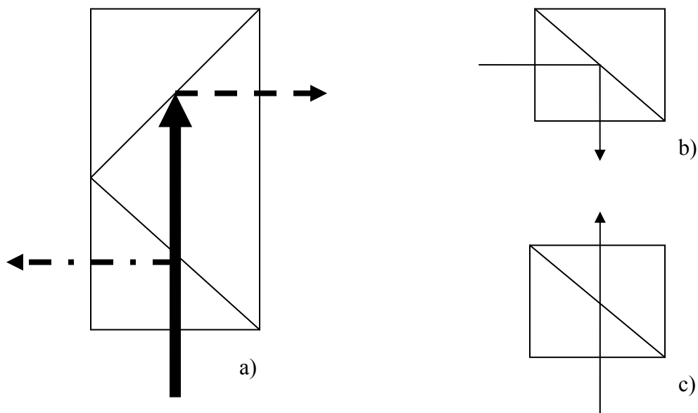
Figure 2.15. a) A PBS which divides the signal into two components. A PBS may also completely b) reflect or c) transmit light depending on the polarization. [10]
