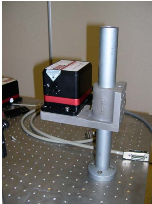
Figure 3.2. The New Focus Velocity diode laser operates through a range of 848nm to 854nm. It was mounted above the table to alleviate the need for multiple periscopes.
