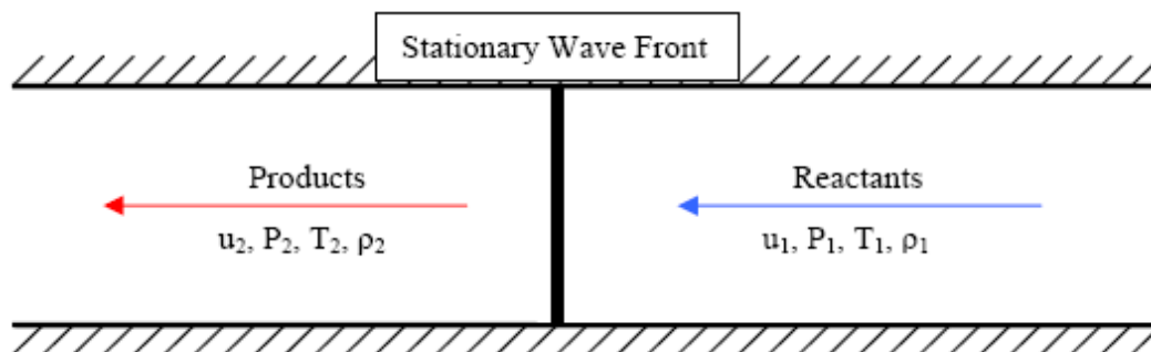
Figure 6. Schematic of stationary combustion wave
