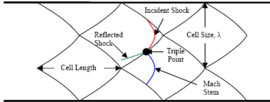
Figure 12. Idealized two-dimensional representation of a detonation's cell structure
