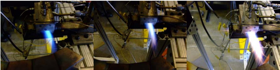
Fig. 60. UCC flames, \phi = 0.7, 1.0, and 1.6 (air ratio = 3.5, fuel = 0.0299 kg/min, airflow varied)
