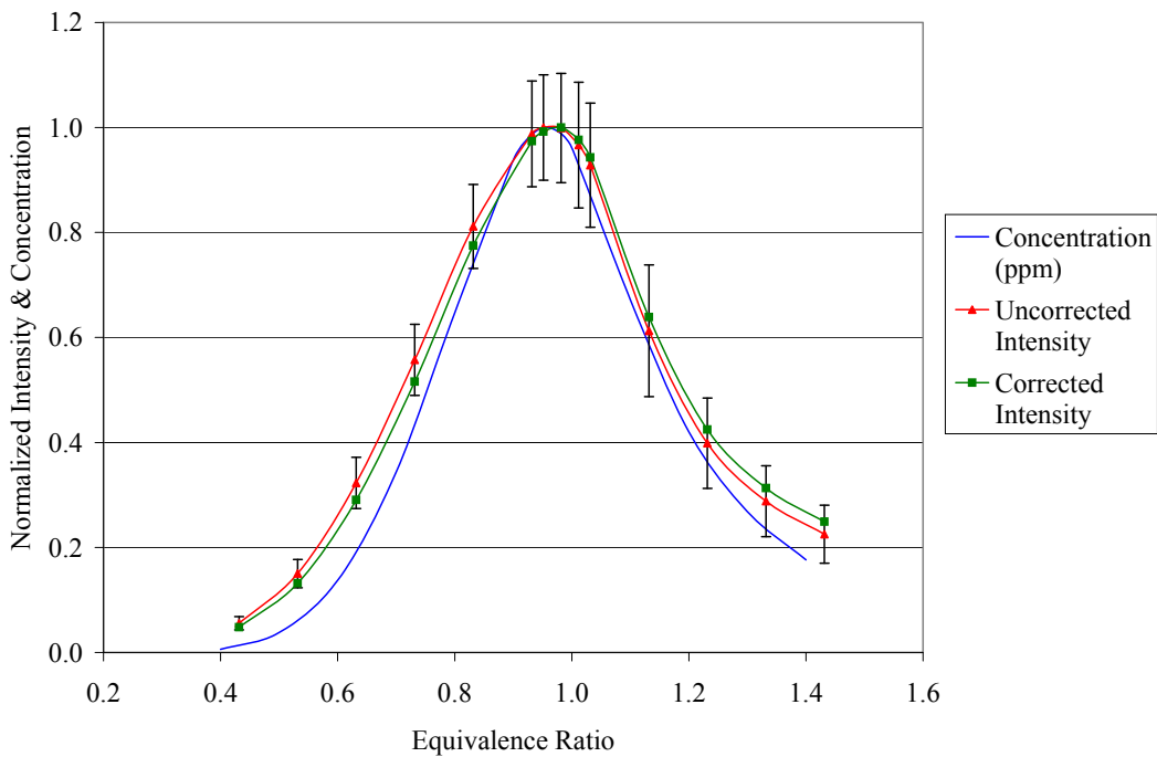
Fig. 43. OH intensities from surface and equilibrium OH concentration
