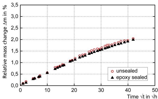
Figure 10: Water absorption behaviour of remote fibre laser cut CFRP [0/90 z /0] s
