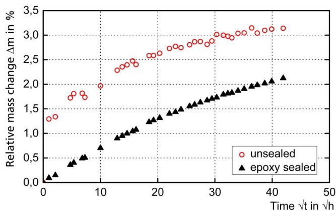
Figure 8: Water absorption behaviour of remote CO 2 laser cut CFRP [0/90 z /0] s
