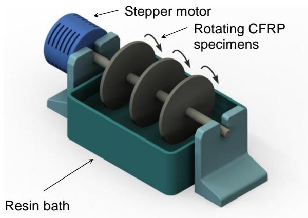
Figure 1: Rotary device for constant resin application conditions
