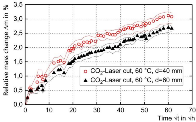
Figure 5: Effect of the specimen diameter d on the water absorption behaviour of remote CO 2 laser cut CFRP [0/90 2 /0] s with different sample diameters d
