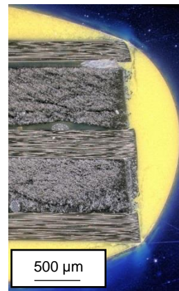
Figure 11: Remote fibre laser cut CFRP edge with yellow sealant
