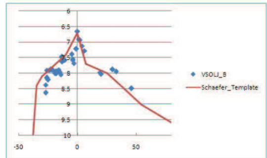
Figure 2: Light curve obtained by VSOLJ members during 2011 outburst.
