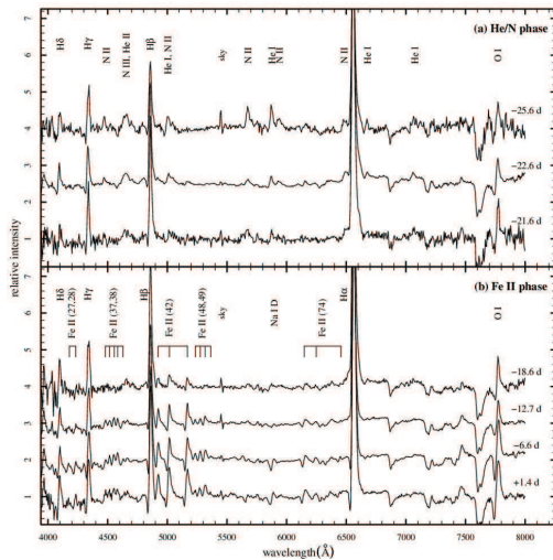
Figure 1: Spectral evolution of T Pyxidis. Upper panel denotes earlier stage, which shows He/N feature. On the contrary lower panel is later stage that shows typical FeII spectral phase. The date after maximum light (minus means before maximum) are denoted on the right shoulder on each spectrum.
