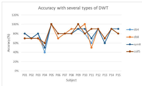
Fig. 3. Accuracy With Several Types of DWT.
