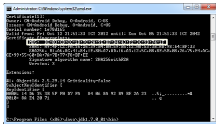
Gambar 3. Generate MD 5
