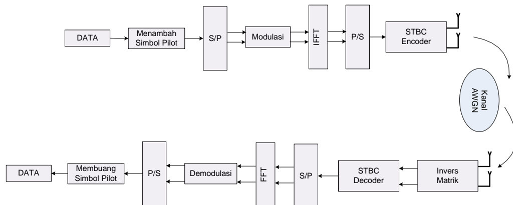
Gambar 2. Blok Diagram Proses Kinerja MIMO-OFDM [1],[3]
