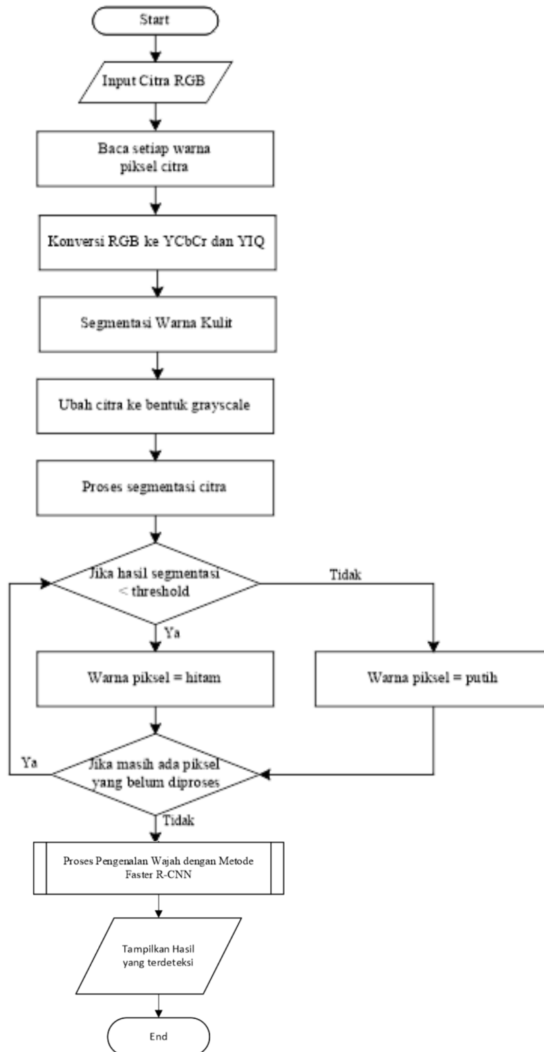
Gambar 1 Flowchart Analisis Proses Pendeteksiian Objek
