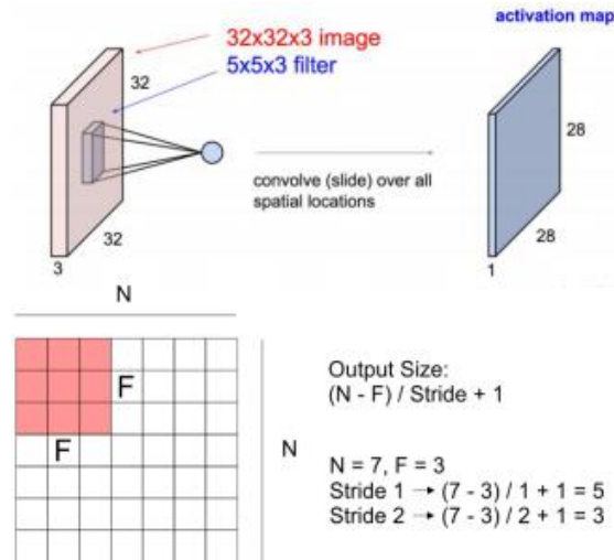
Gambar 3 Convolutional Layer [6].
