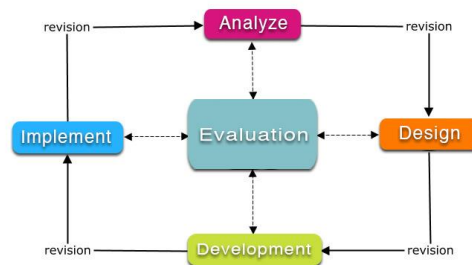
Gambar 4. ADDIE Model
