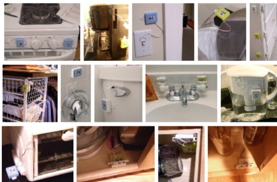
Figure 2.17: Some of the 77 “tape of forget” sensors deployed in a house in [Tapia et al., 2004].
