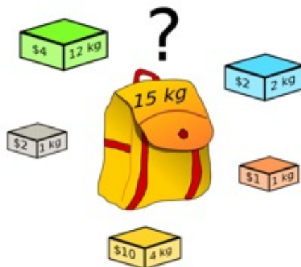
Figure 2.6: The knapsack problem.
