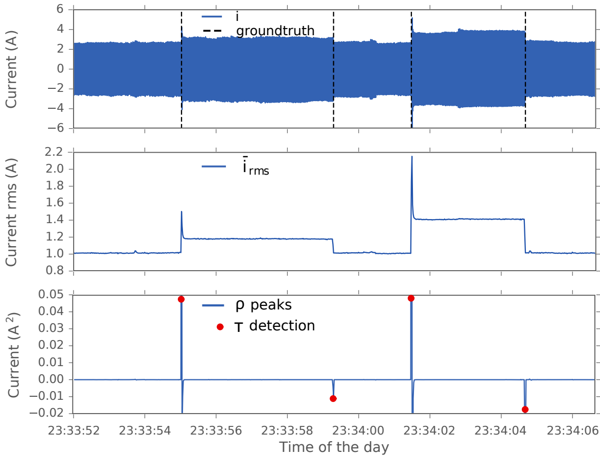
Figure 4.2: Illustration of the event detection algorithm. (a) i Current waveform from the mains and ground-truth of events; (b) Envelope extraction: \bar{i}_{rms} normalized rms value for the current; (c) \rho peak signal and \tau event detection.
