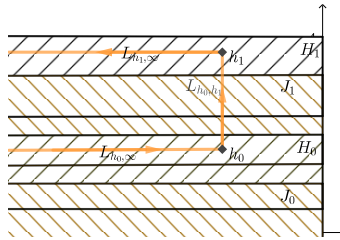
FIGURE 2. Integration path for the difference of solutions
