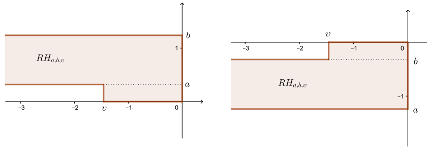
FIGURE 5. Sets RH_{a,b,v} = H \cup R_{a,b,v}
