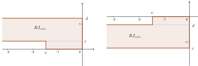
FIGURE 6. Examples of sets RJ_{c,d,v} = J \cup R_{c,d,v}
