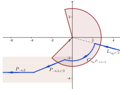
FIGURE 4. Deformation of the integration path
