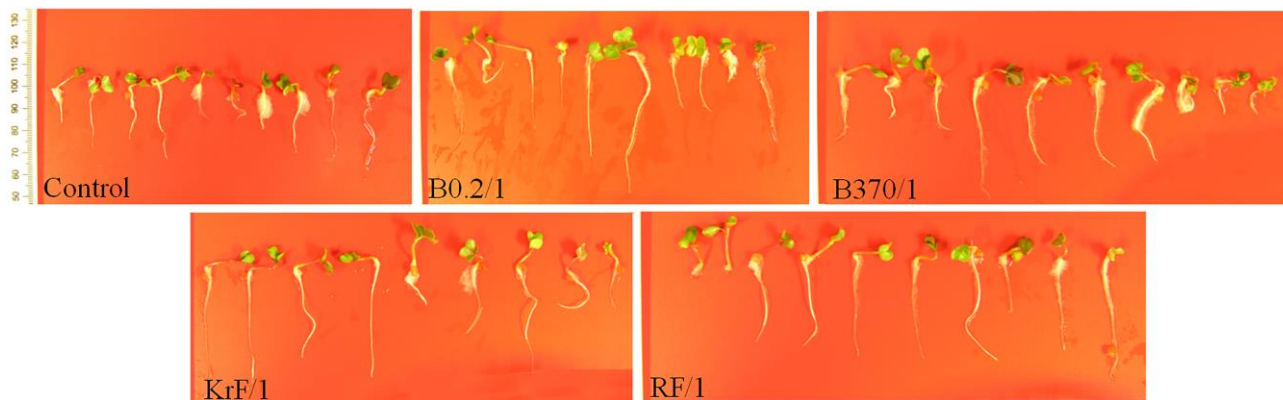
Fig. 5. Seedlings from seeds untreated (control); seedlings from seeds exposed to magnetic field at 0.2 Hz (B0.2/1), to magnetic field at 370 kHz (B370/1), to radiofrequency at 900 MHz (RF/1) for 120 h and to laser (excimer laser) KrF/1 at 248 nm for 30 kshots .
