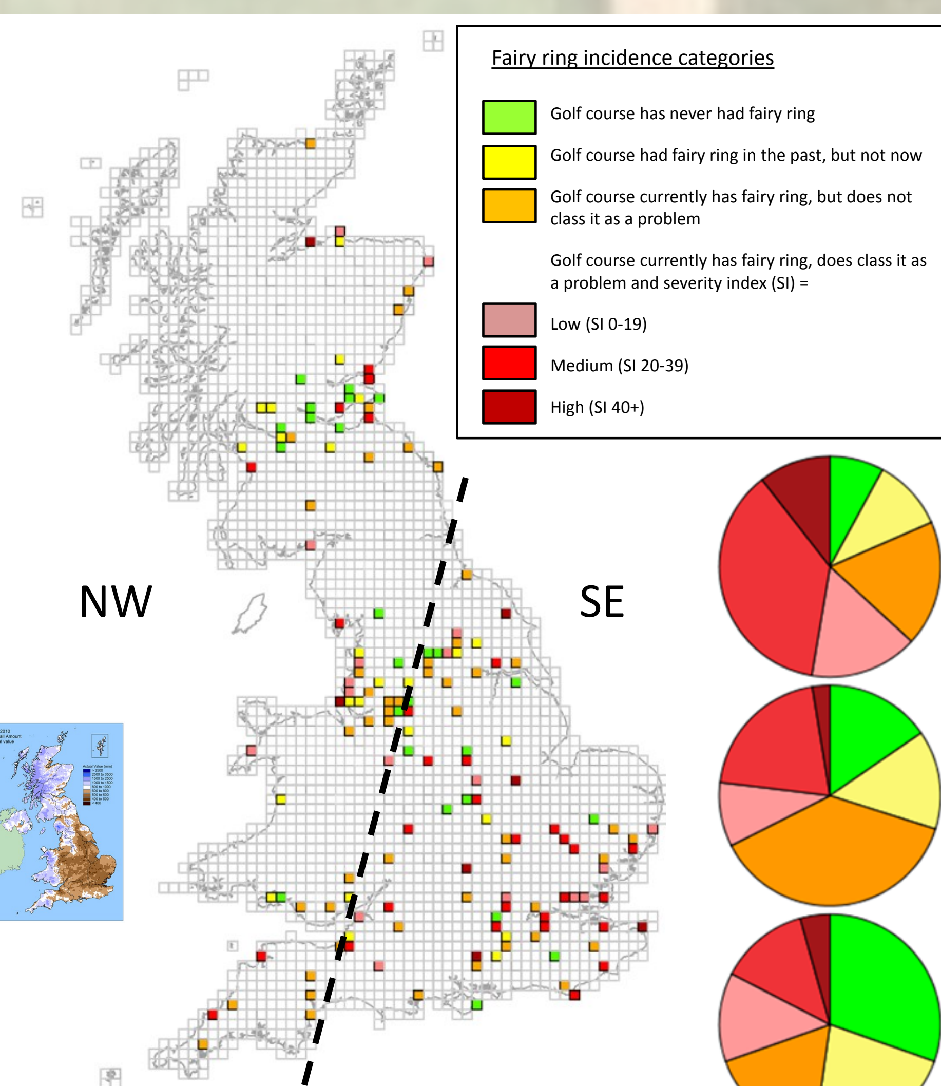
Figure 5: Map of fairy ring incidence on UK golf courses. Inset: UK MetOffice map of annual rainfall demonstrates the climatic divide seen between the north and west (NW) and south and east (SE) of the country. A line intersected across the incidence map to represent this divide allows for comparison by climatic region.
