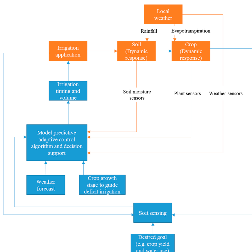
Figure 1. Conceptual model-based decision support system for precision irrigation. Elements in blue represent novel ideas from the Authors and elements in orange are from the decision support system presented in McCarthy et al. [114].
