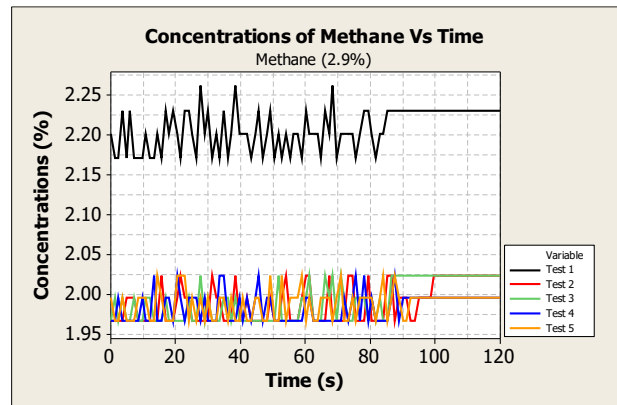
Figure 10: Graph of CH 4 concentrations (2.9%) versus time
