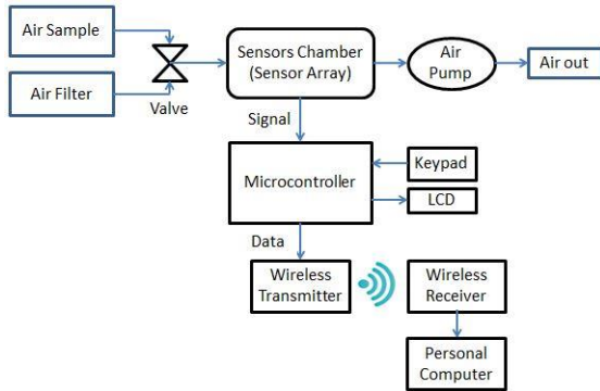
Figure 1: General e-nose system
