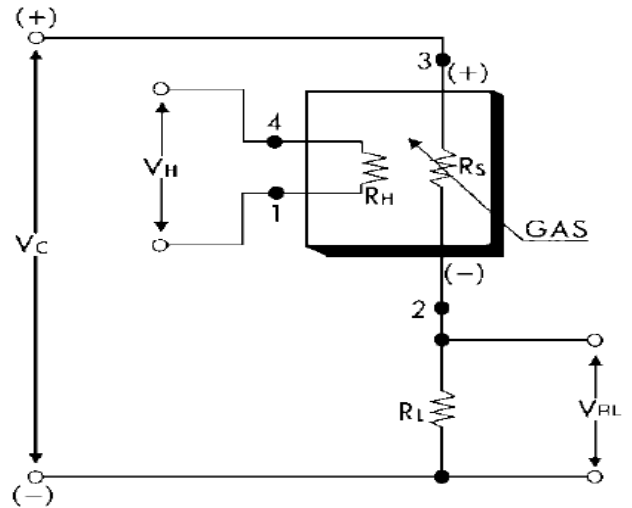
Figure 4: MOS gas sensor circuit diagram
