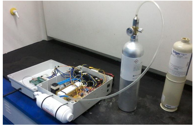
Figure 6: The e-nose in a fume hood for gas exposure
