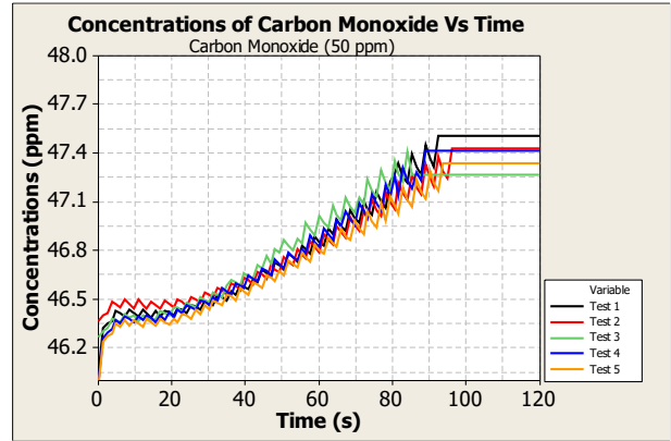
Figure 9: Graph of CO concentrations (50 ppm) versus time
