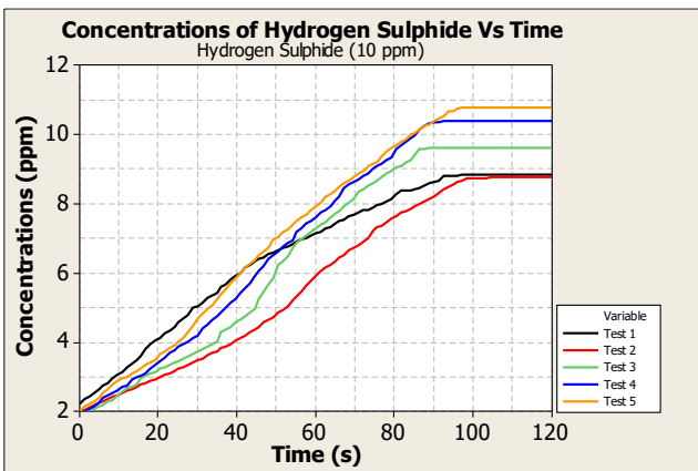
Figure 8: Graph of H 2 S concentrations (10 ppm) versus time
