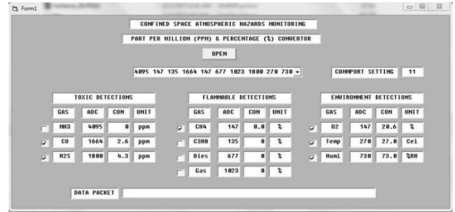
Figure 3: Graphic User Interface (GUI)
