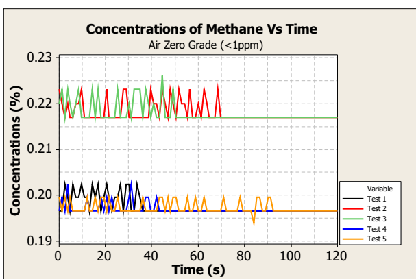
Figure 13: Graph of CH 4 concentrations (<1 ppm) versus time
