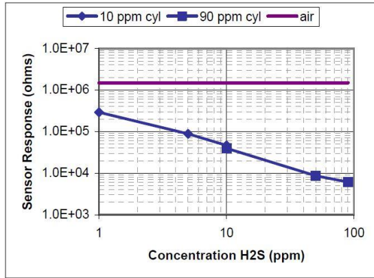
Figure 5: Graph of hydrogen sulphide (H 2 S) sensor response versus concentrations
