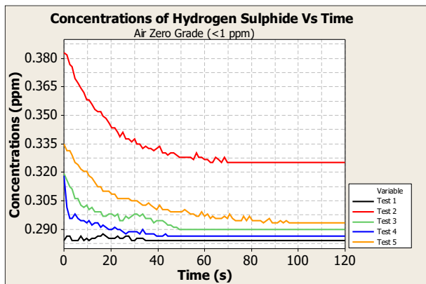
Figure 11: Graph of H 2 S concentrations (<1 ppm) versus time
