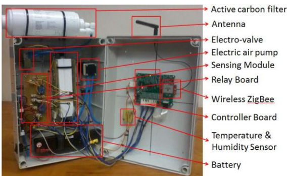
Figure 2: E-nose full hardware development
