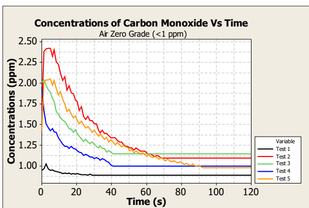
Figure 12: Graph of CO concentrations (<1 ppm) versus time
