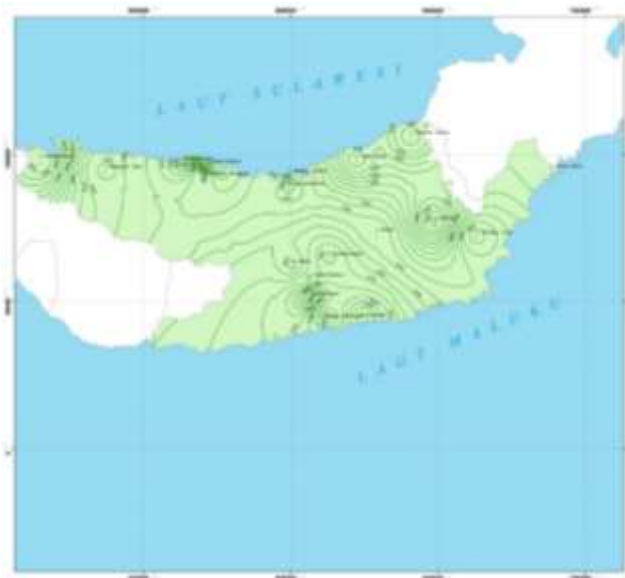
Gambar 6. Peta Isohyet WS Dumoga Sangkub
