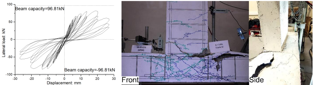
(a) Specimen JB-2T-E00
