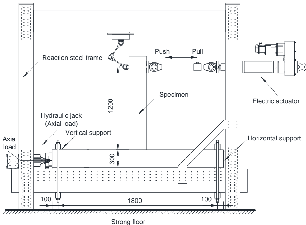
Fig. 2 Test set-up
