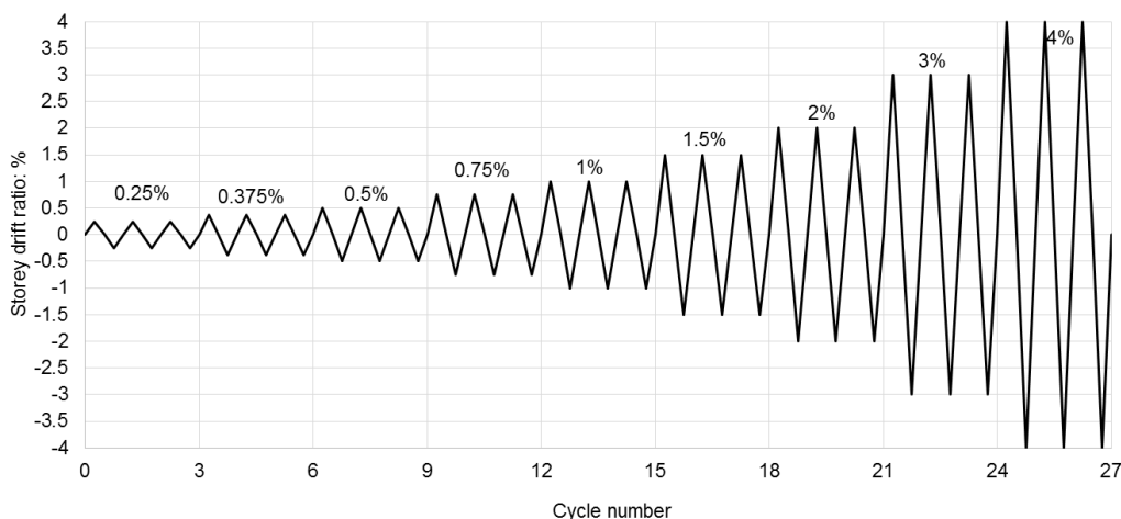
Fig. 3 Loading history
