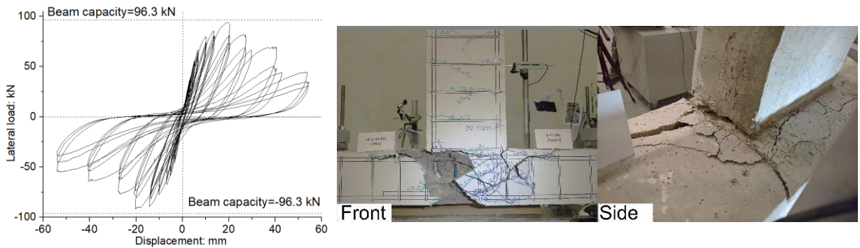
(b) Specimen JB-0T-E75
