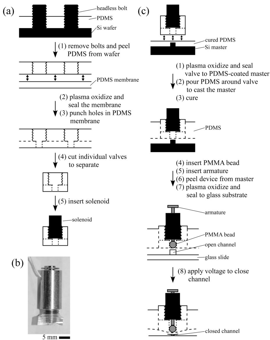
Fig. 3. Fabrication of solenoid valves. (a) Prefabrication of the solenoid valve. First, we created an array of PDMS nuts by molding PDMS around headless bolts. We sealed the array of PDMS nuts to a thin (1 mm) membrane of PDMS and punched 1.5-mm holes through the membrane, such that the holes were concentrically aligned with the PDMS nuts. Individual valves could be separated with a razor blade. It was possible to insert a cylindrical solenoid with into each PDMS structure. Solenoids were approximately 10 mm in diameter, and 24 mm in height, with external threads along the lower 6 mm of the casing of each solenoid. (b) A photograph of a prefabricated solenoid valve. (c) Incorporation of the prefabricated solenoid valve into a microfluidic device. We spin-coated a layer of PDMS onto the silicon master. After curing this layer of PDMS, we manually sealed the valve to the master directly above an SU-8 channel. The device was then molded in PDMS and cured. The dashed lines indicate the fusion of different layers of PDMS. Once cured, the devices were removed from the master, plasma oxidized, and sealed to a glass slide. A PMMA bead, 1.5 mm in diameter, was dropped through the center of the solenoid, and the armature of the solenoid
