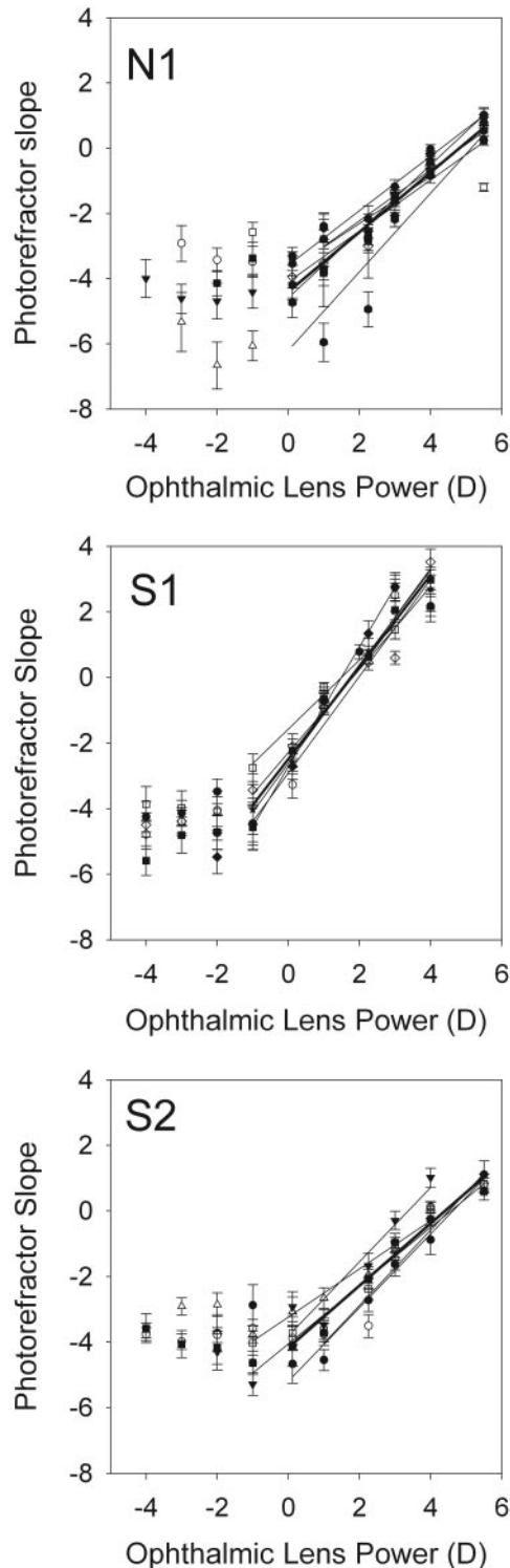
FIGURE 3. Panels show calibration curves developed on different experimental days in normal (N1) and strabismic (S1 and S2) monkeys. The average calibration curve is shown by the darker line in each of the panels.
