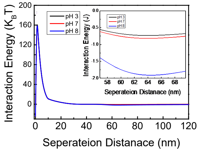
2 Figure 6. DLVO interaction for synthetic produced water under various pH (a) Interaction energy of 3 oil droplets in 25 ppm of synthetic produced water prepared by oil at API 24.3. (b) Interaction energy 4 of oil droplets in 25 ppm of synthetic produced water prepared by oil at API 36.3.
