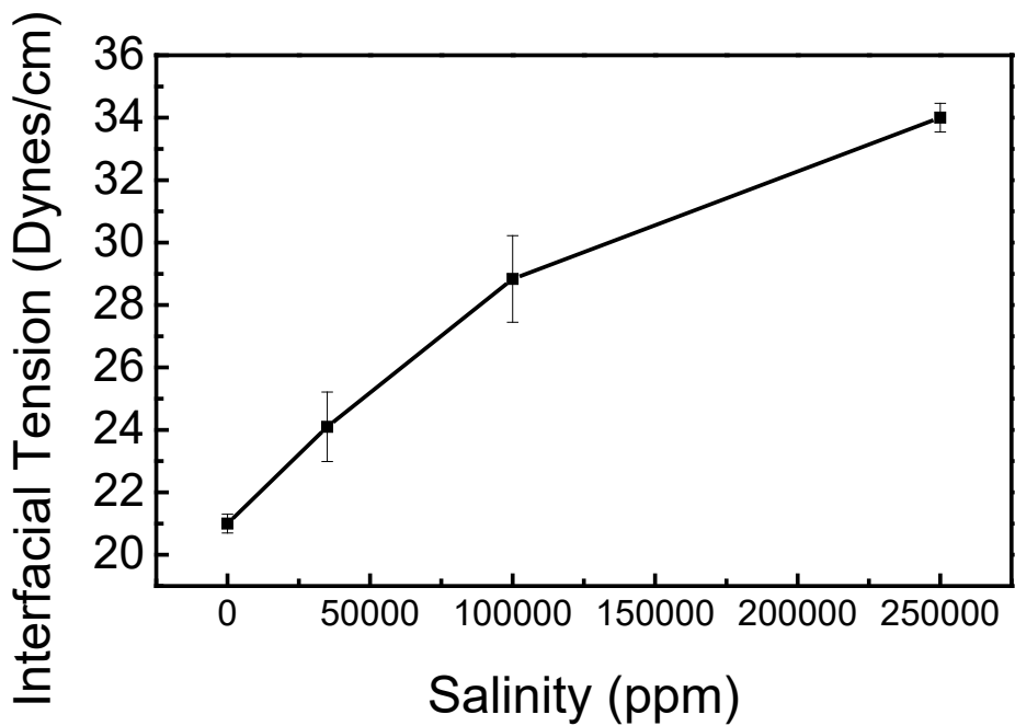
8 Figure 3. Interfacial tension between saline water at zero, 35000, 100000, and 250000 ppm of salt 9 concentration and oil with API 36.3.
