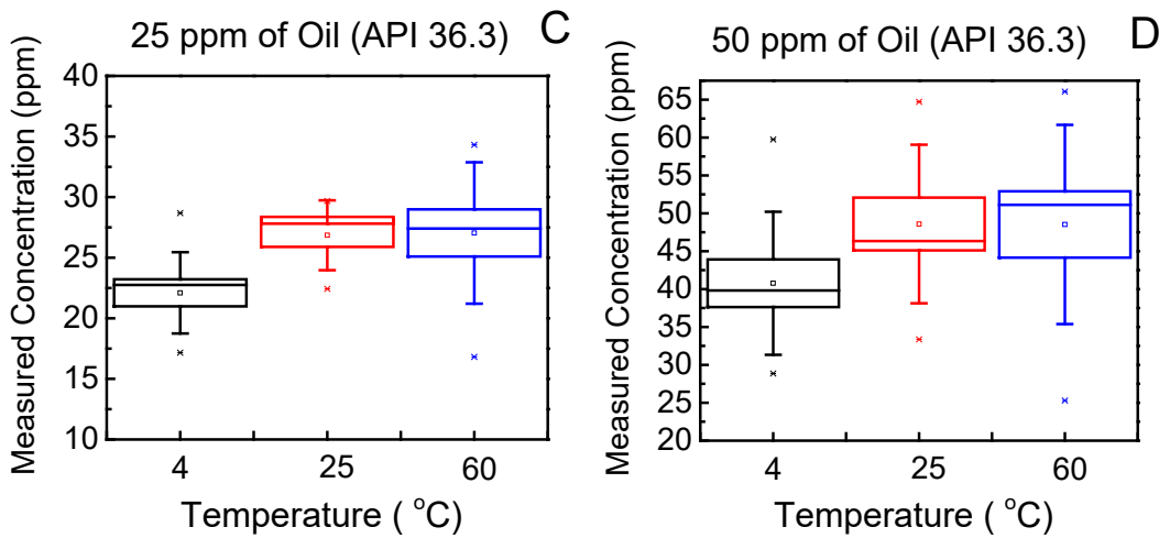
3 Figure 7. CLFM measurements for produced water prepared with crude oils with different API 4 values under different temperature. The dot inside the box represents the mean value, and the line 5 inside the box represents the median value in the dataset. The box is plotted by mean \pm standard 6 error, and the whisker is plotted by mean \pm standard deviation.
