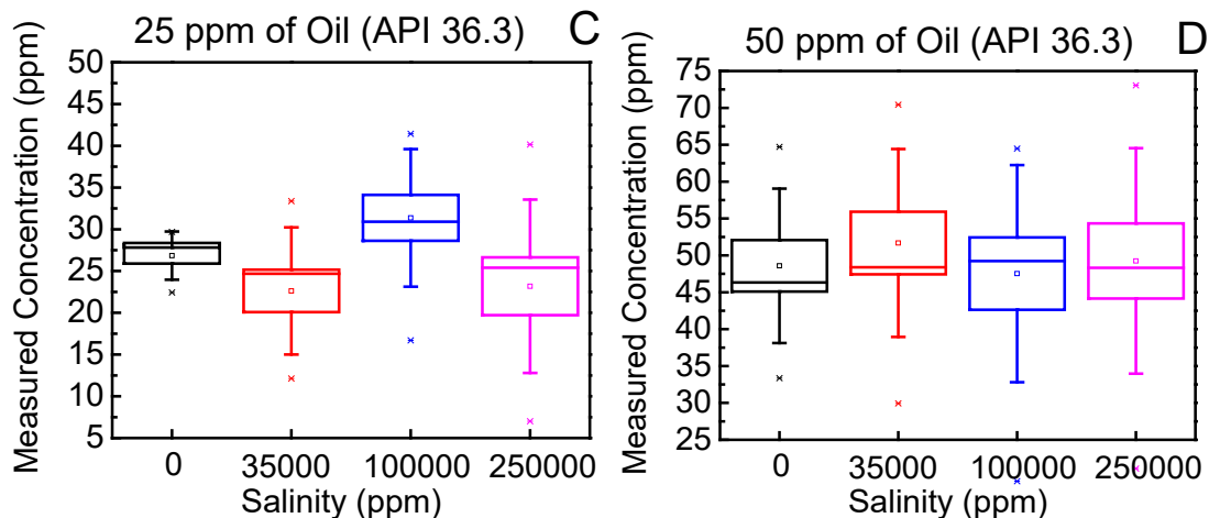
1 2 Figure 1. CLFM measurements for produced water prepared with crude oils with different API 3 values (API 24.3 – heavy oil and API 36.3 -light oil). The dot inside the box represents the mean 4 value, and the line inside the box represents the median value in the dataset. The box is plotted by 5 mean \pm standard error, and the whisker is plotted by mean \pm standard deviation. The dots outside 6 the boxes and whiskers are data beyond the range of mean \pm standard deviation. 7
