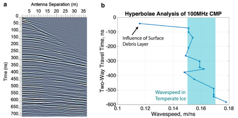
Fig. 3. Common midpoint survey used to determine radio wave speed in the subsurface. (a) Common midpoint radargram. (b) Velocities resulting from common midpoint hyperbolae analysis. Mean velocity = 0.156 \text{ m ns}^{-1} , a value consistent with temperate glacial ice.
