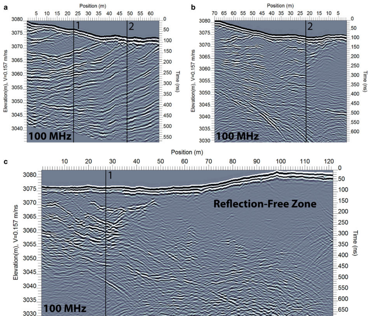
Fig. 5. 100 MHz radargrams acquired on the east side of the cirque. (a) Flow-parallel profile displaying numerous (>6) strong up-glacier dipping reflectors. North by northeast/downglacier is to the right. (b) Flow-transverse profile displaying complex, broken geometry of reflectors. Northwest is to the right. (c) Flow-transverse profile that extends into the center glacier, illustrating how localized the reflector set is; the main glacier body is for the most part reflection-free. In this view we see the reflectors are concave-up, forming a tight nested-spoons geometry. Numbered black lines in each panel indicate the point of intersection between transects. West by northwest is to the right.
