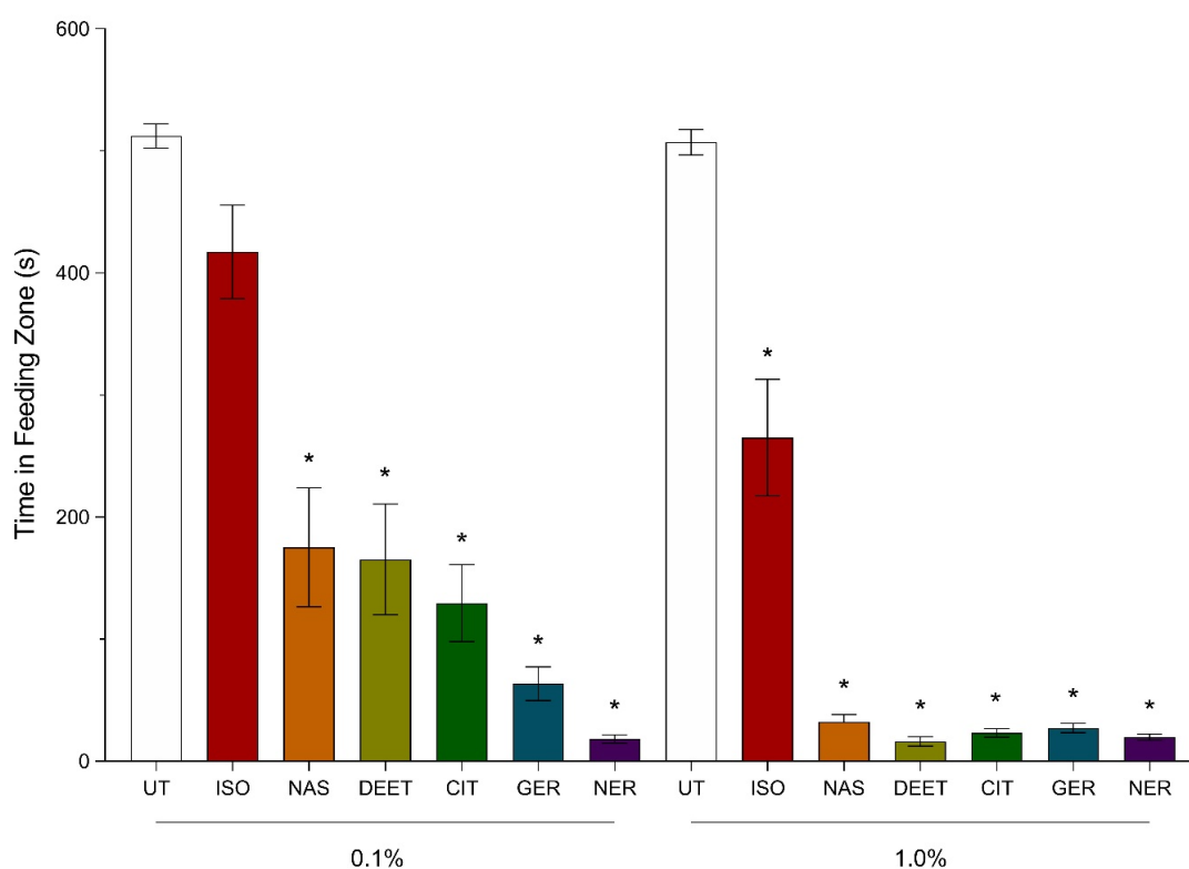
Figure 2. Efficacy of Nasonov terpenoids and N,N -diethyl- meta -toluamide (DEET) at 0.1 and 1.0% ( v/v ). Untreated (UT), isoamyl acetate (ISO), synthetic Nasonov pheromone (NAS), citral (CIT), geraniol, (GER), and nerol (NER). A video tracking protocol with individual bees in Petri dishes was used to observe behavior changes when exposed to sugar–agarose cubes treated with the terpenoids. The UT controls were sugar–agarose cubes with no terpenoid or DEET treatment. The DEET treated sugar–agarose cubes were screened as a positive control. Vertical bars represent mean ± standard error. Asterisks above the bars indicate a significant difference between the mean of the terpenoid- or DEET-treated bees compared to the UT bees using a one-way ANOVA with a Tukey’s post-hoc test ( p < 0.0001 ).
