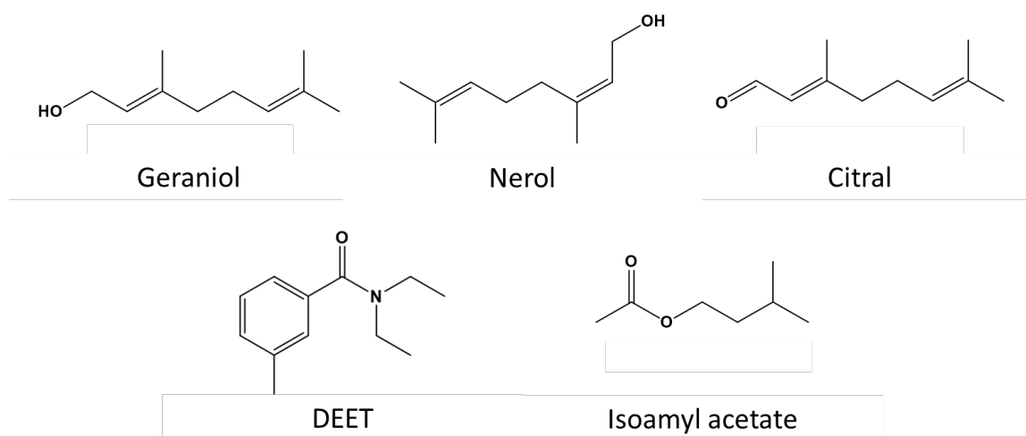
Figure 1. Chemical structures for the Nasonov terpenoids (geraniol, nerol, and citral), N,N -diethyl-meta-toluamide (DEET), and isoamyl acetate.
