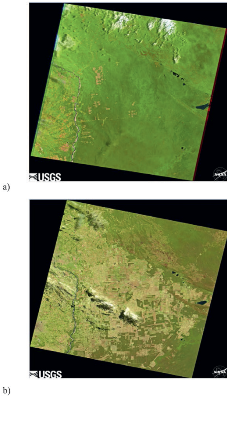
FIG. 2. LULCC in the Amazonian central Bolivia observed by Landsat satellite: (a) intact forests (green) prior to deforestation (light color) on 7 Nov 1986 and (b) after deforestation on 29 Aug 2013. Each image is 185 km × 185 km. The river on the western side of the images is the Rio Grande O Guapay, an upper tributary of the Amazon River.
