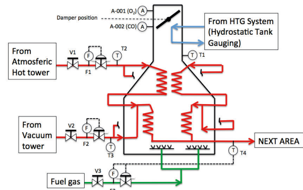
Fig. 3. Vacuum oven
