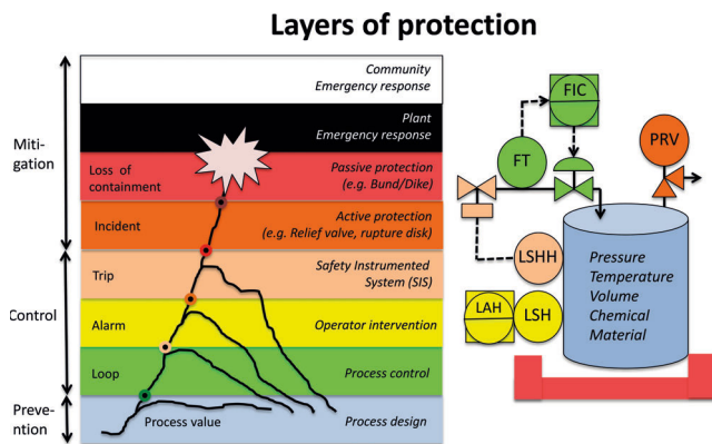
Fig. 1. Safety layers of protection
