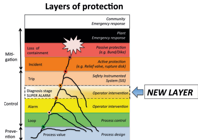
Fig. 2. "Super alarm" layer of protection
