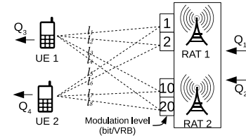
Fig. 5. Example with 2 RATs, 2 users, 2 available modulations per RAT and user. Queues Q_1/Q_3 and Q_2/Q_4 are respectively incoming/outgoing queues for user 1 and 2. Links \{l_1 \dots l_8\} connect all queues in the system according to incidence matrix shown in Eq. (1), i.e., allowing different amount of bits per slot (different modulation levels), i.e., m_{1,1,1} = m_{1,2,1} = 1 bit/slot and m_{1,1,2} = m_{1,2,2} = 2 bits/slot (from RAT 1 to user 1 and 2), and m_{2,1,1} = m_{2,2,1} = 10 bits/slot and m_{2,1,2} = m_{2,2,2} = 20 bits/slot (from RAT 2 to user 1 and 2).
