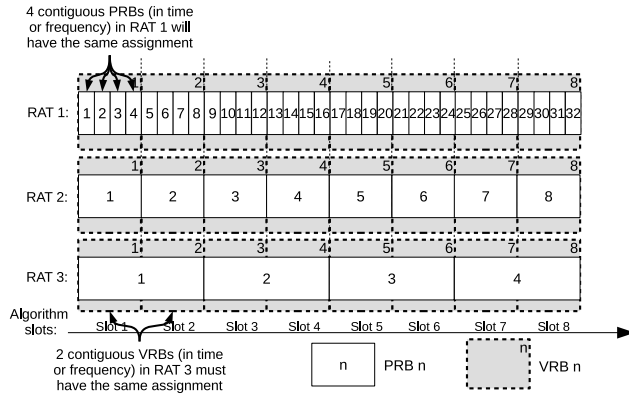
Fig. 6. Three RATs with capacity 32, 8, and 4 PRBs, respectively, per time×bandwidth, like the example shown in Fig. 3a. One VRB in RAT 1 contains four PRBs with equal allocation. One PRB in RAT 3 contains two VRBs which must have equal allocation.
