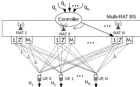
Fig. 4. System model. A network of queues with N incoming queues and N outgoing queues. Our network controller needs to select a RAT and a modulation index (i.e. a link connecting queues) to deliver data between each pair of queues \{Q_i, Q_{N+i}\} .
