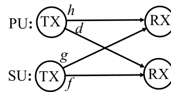
Fig. 1. UCR channel model as a SISO two-user IC.
