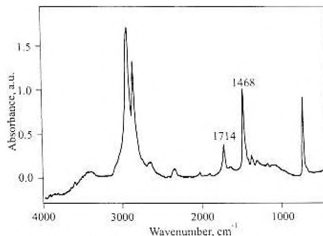
Fig. 1. FT-IR spectrum of C AE sample exploited 4 months
