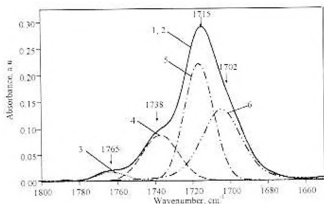
Fig. 2. FT-IR spectra of C_{AE} sample exploited 4 months (see Fig. 1b): 1 — experimental spectrum, 2 — calculated spectrum, 3 — ester band, 4 — aldehyde band, 5 — ketone band, 6 — acidic band. Experimental data and spectrum calculated as a superposition of 4 sub-bands
