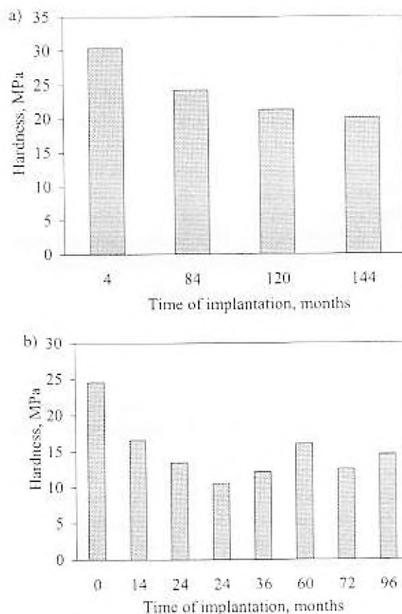
Fig. 4. The dependence of hardness on the time of implantation PE samples: a) C_{AE} , b) C_{II}
