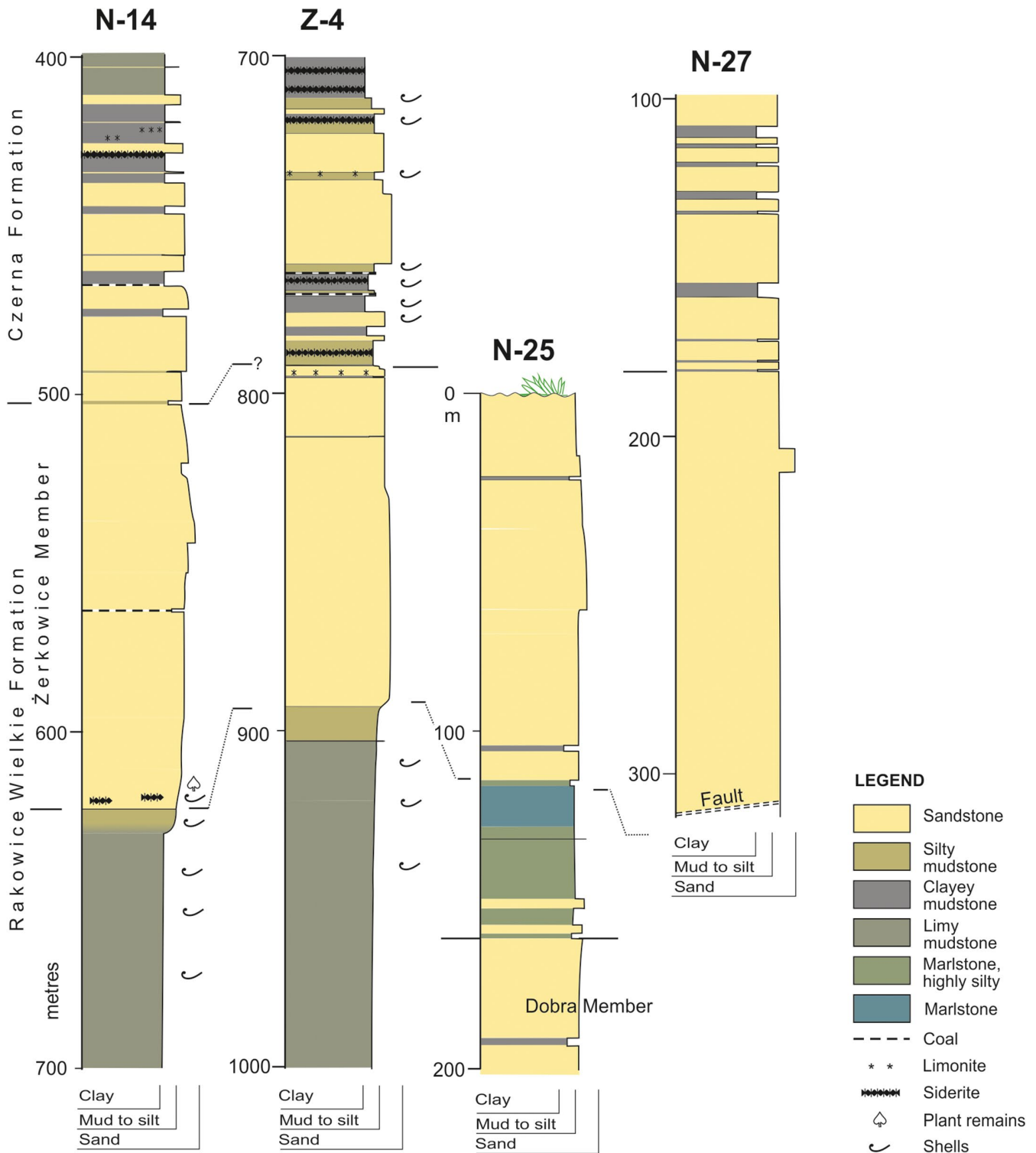
FIGURE 3 Borehole logs showing the stratigraphic transition of the Rakowice Wielkie Formation to the Czarna Formation; for borehole location, see Figure 1B. Log N-14 is based on Bossowski et al. (1976) and Bossowski (1991a); log Z-4 on Kochanowska (1988) and Leszczyński (2018); log N-25 on Dyja (1978) and Bossowski et al. (1978); and log N-27 on Bossowski et al. (1977)
