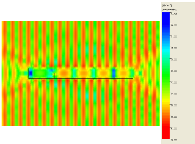
Figure 13. Simulated electric field distribution for 2 GHz.
