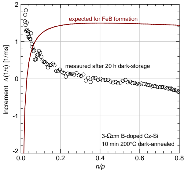
Figure 10. Increment in the reciprocal lifetime \Delta(1/\tau) induced by a 20 h dark storage of the historic sample preannealed in the dark at 200 °C for 10 min (circles). The solid curve is a scaled calculated increment due to the pairing of Fe into FeB.
