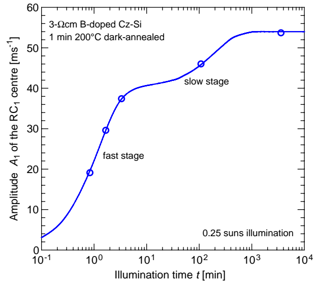
Figure 6. Evolution of the amplitude A_1 of \text{RC}_1 as deduced from the curves shown in Figure 5 using Equation (2). The solid blue line is the double-exponential fit of Equation (3) to the measurement data shown as open circles. The time constants extracted from the fit are t_f = 1.25 min for the fast and t_s = 200 min for the slow stages.
