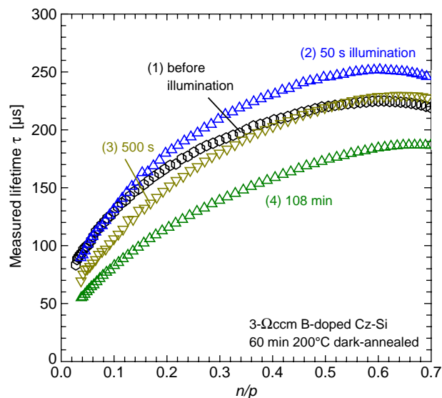
Figure 9. Measured effective lifetime \tau as a function of n/p for the historic 3 \Omega\text{cm} boron-doped Cz-Si sample of Figure 4, preannealed in the dark at 200 °C for 60 min and then illuminated at T_{\text{room}} at a light intensity of 0.25 suns. The curves 1–4 are for different illumination times: (1) before illumination (0 s), (2) 50 s, (3) 500 s, and (4) 108 min, respectively.
