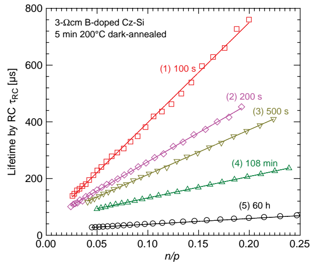
Figure 7. Injection-level dependence of the lifetime by the illumination-induced RC \tau_{\text{RC}} calculated by Equation (1) for the historic 3 Ωcm boron-doped Cz-Si sample of Figure 4, preannealed in the dark at 200 °C for 5 min and then illuminated at T_{\text{room}} , at a light intensity of 0.25 suns. The curves 1–5 are for different illumination times: (1) 100 s, (2) 200 s, (3) 500 s, (4) 108 min, and (5) 60 h, respectively.
