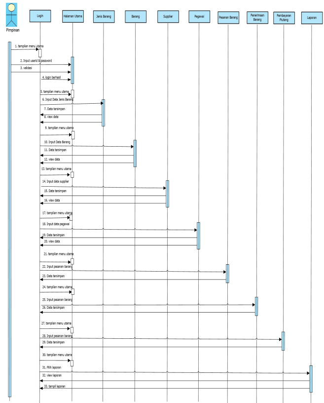
Gambar 4. Squece Diagram Actor Pimpinan
