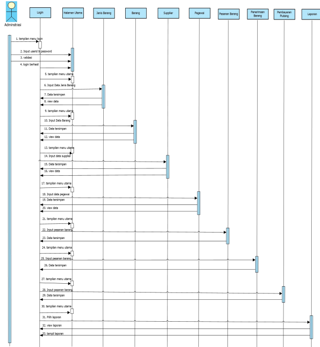
Gambar 5. Squen Diagram Actor Administrasi
