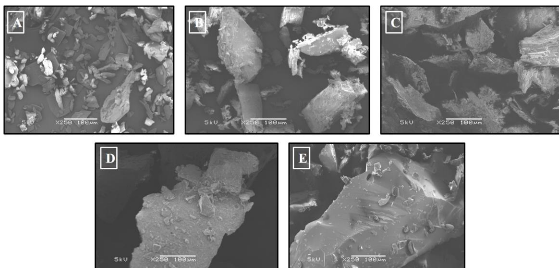
Figure 6 Scanning electron microscopy images of (A) Indo, (B) Tro, (C) 1:1 Indo-Tro crystalline salt prepared by SE, (D) 1:1 Indo-Tro crystalline salt prepared by HME and (E) 1:1 Indo-Tro amorphous product prepared by HME.
