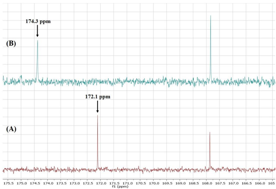
Figure 12 ^{13}\text{C} NMR of (A) Indo and (B) 1:1 Indo-Tro crystalline salt prepared by HME.
