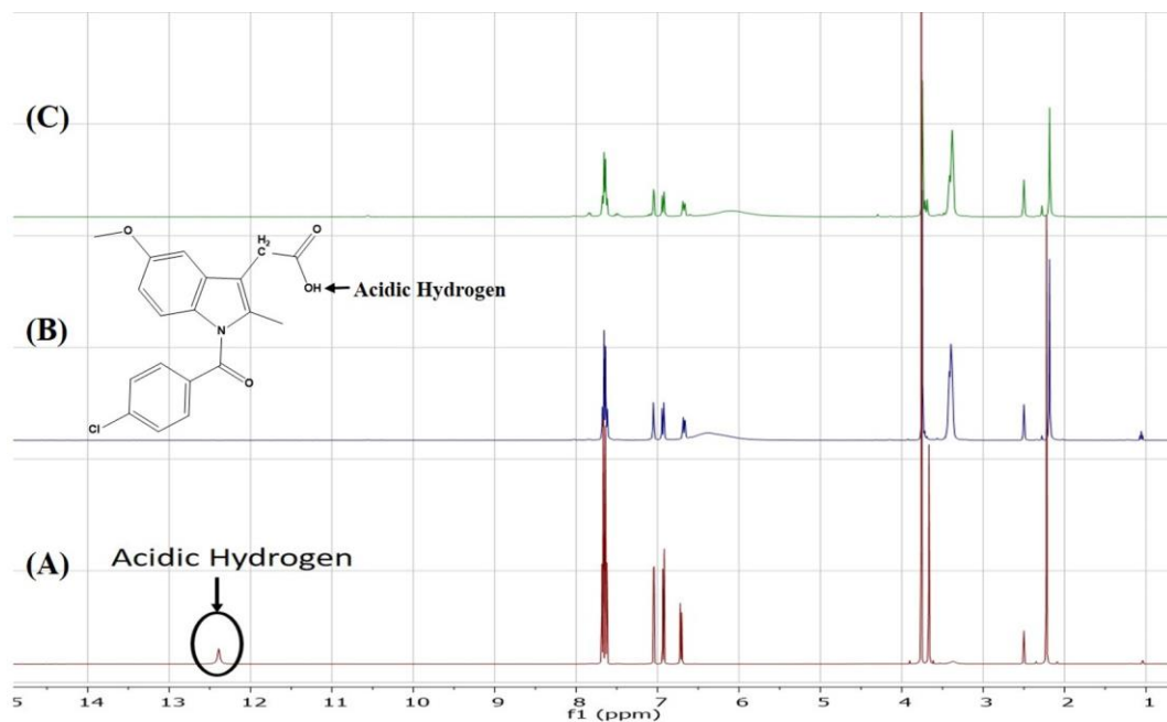
Figure 11 ^1\text{H} NMR of (A) Indo, (B) 1:1 Indo-Tro crystalline salt prepared with SE and (C) 1:1 Indo-Tro crystalline salt prepared by HME.
