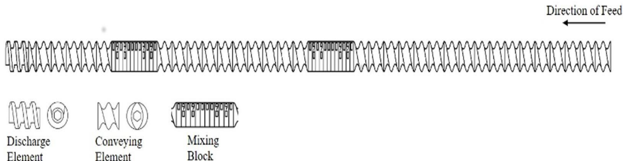
Figure 1 Illustration of ideal screw configuration used in HME.
