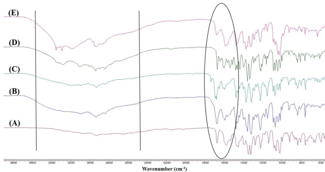
Figure 8 FTIR spectra of (A) Indo, (B) Tro, (C) 1:1 Indo-Tro crystalline salt prepared by SE, (D) 1:1 Indo-Tro crystalline salt prepared by HME.
