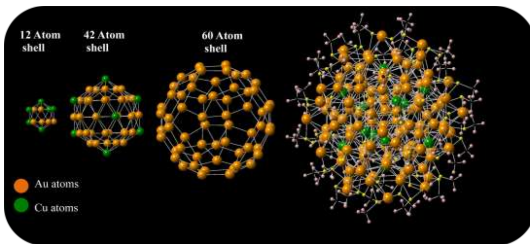
Figure 12. Cu atoms are interdispersed in Au 12 and Au 42 shells of Au 144 (SR) 60
