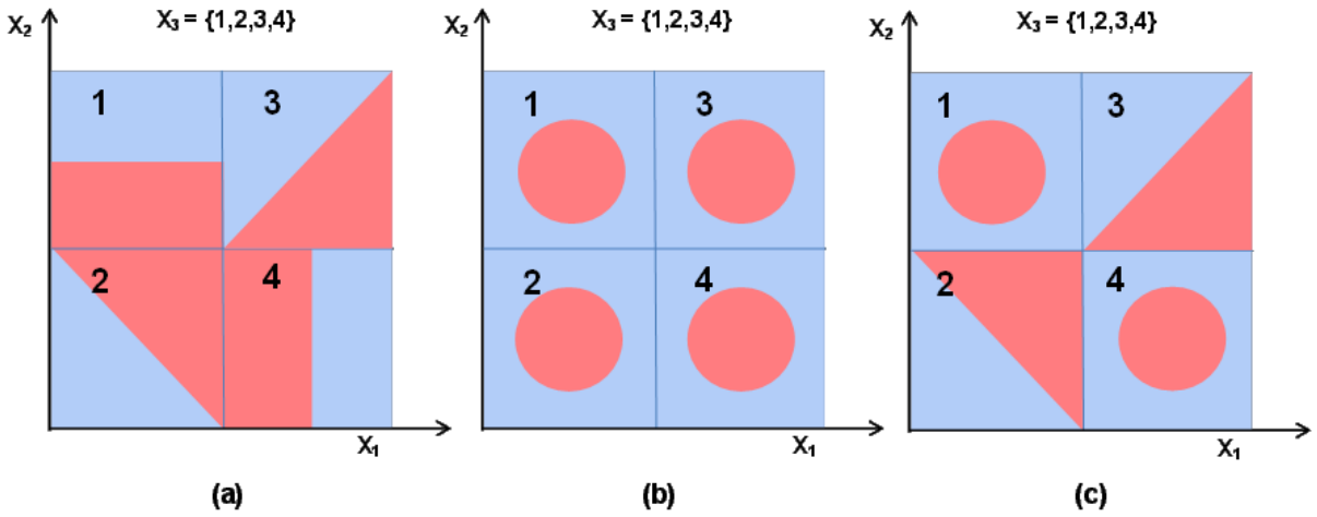
Figure 3.1. Examples of Piece-wise Separable Classification Problems.
