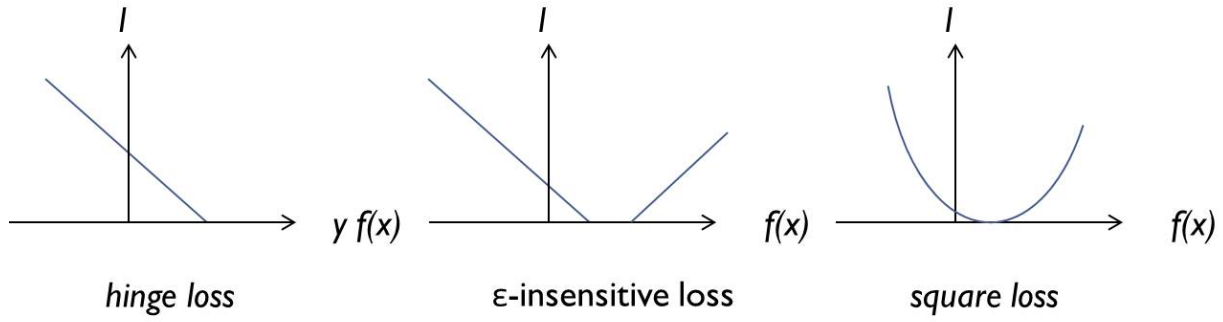
Figure 2.2. Loss function comparison
