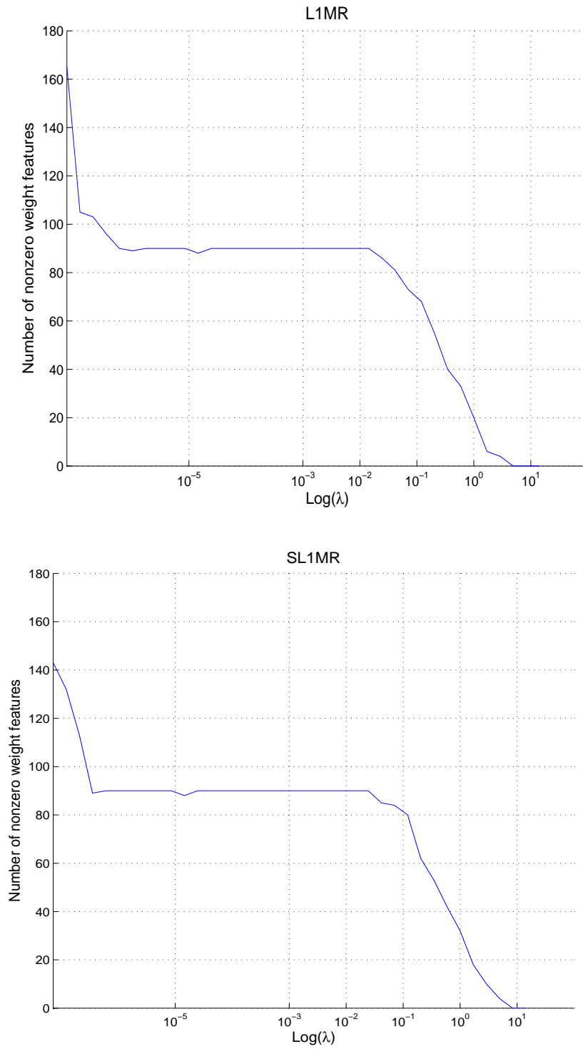
Figure 2.5. The relationship between \lambda and the number of non-zero-weight features.
