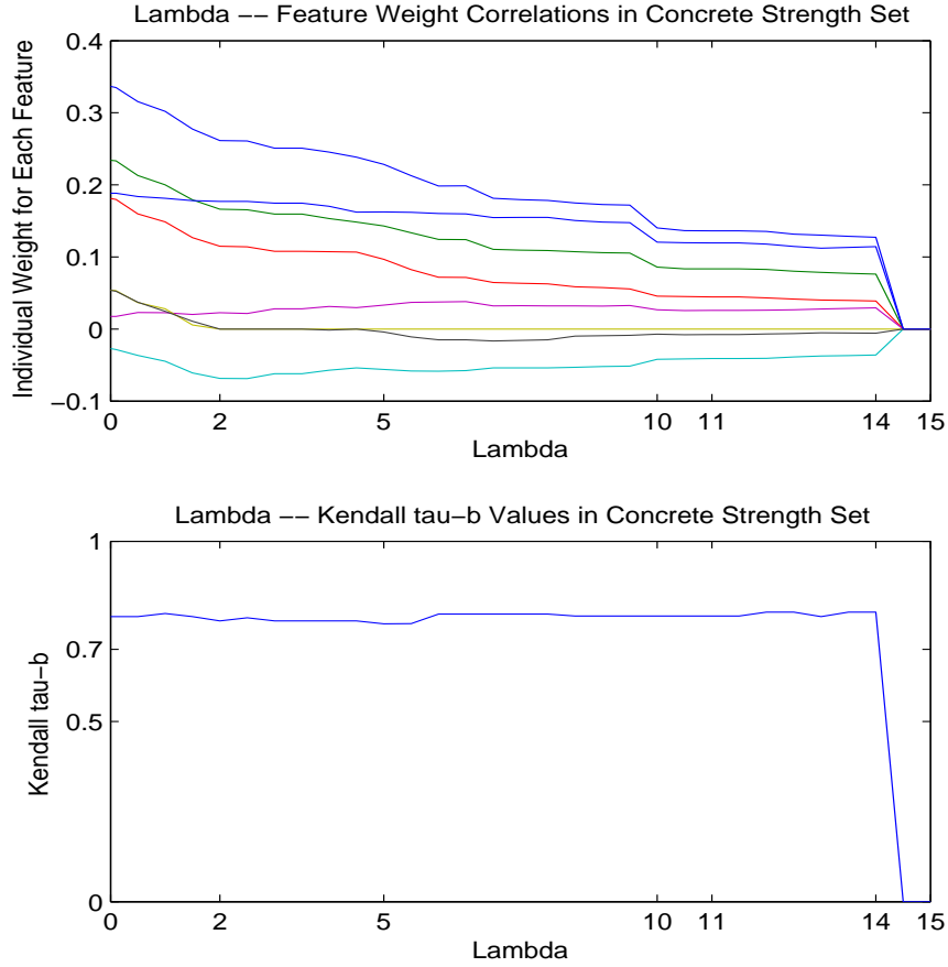
Figure 2.4. The relationship between \lambda , feature weights ( w_j 's), and Kendall \tau -b rank correlation coefficient on the Concrete Strength data set.
