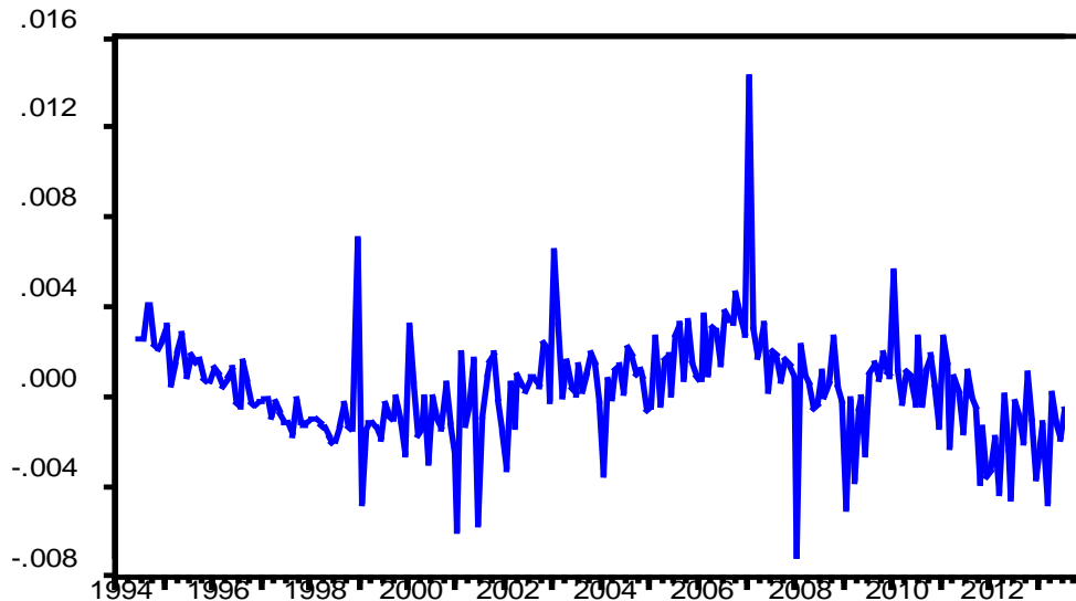
Figure 3: Cointegration Graph
