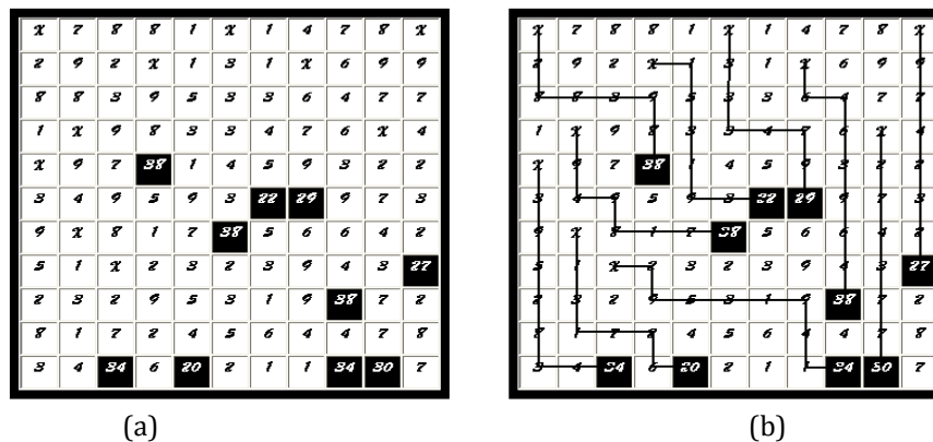
Figure 4: An example of a 11 X 11 Speed++™ puzzle (a) with its solution (b)
