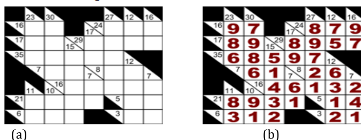
Figure 1: An example of a Kakuro puzzle (a) with its solution (b) (Wikipedia – Kakuro, 2012)
