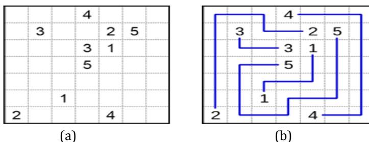
Figure 2: An example of a Numberlink puzzle (a) with its solution (b) (Wikipedia – Numberlink, 2012)
