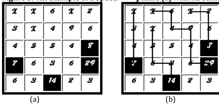
Figure 3: An example of a Speed++™ puzzle (a) with its solution (b)
