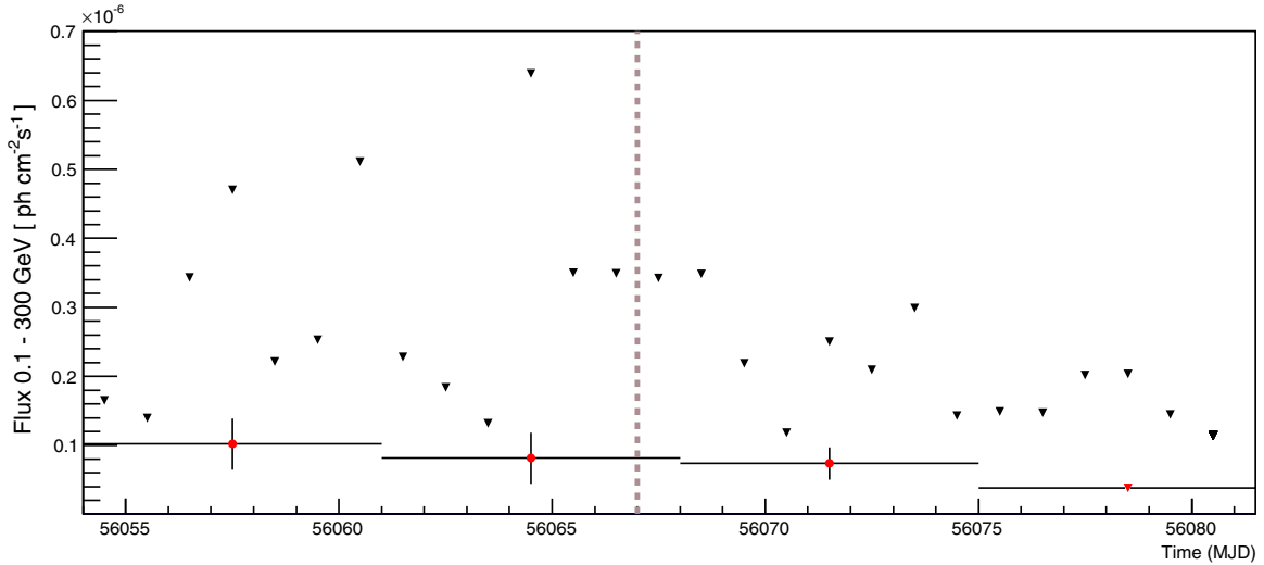
Figure 4. High-energy gamma-ray light curve of 1ES 1959+650 as observed by Fermi LAT. Analysis is completed over four weeks on both a daily and weekly bases from MJD 56054 through MJD 56082. Upper limits are calculated from epochs where the TS value is less than 9, which was every day in the four-week window, as well as the bin corresponding to the last week. There is no indication of detected high-energy gamma-ray variability during this time period. The time corresponding to the elevated state of the VHE data is highlighted by the gray dotted line. (A color version of this figure is available in the online journal.)
