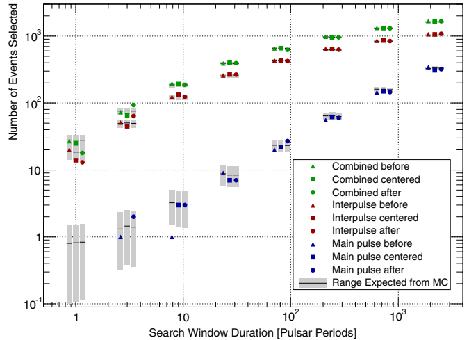
Figure 6. Number of gamma-ray events selected (symbols) vs. the duration of the search window. The gray regions denote 68% containment intervals about the mean of the distribution (black line) determined from searches performed on the Monte Carlo data. The Monte Carlo data set is composed of 500 simulated time series containing an injected signal from the Crab pulsar at the level of the measured VHE pulsar flux ( x_i = 1 ). The absence of a symbol in four of the searches indicates that the number of selected events in each of these cases was zero. All searches return values which are consistent with what is found from searches on the Monte Carlo data sets. The slight negative and positive shift of the x -position of the before and after symbols is done as a visual aid to prevent clutter about the common x -coordinate value for the before , centered , and after symbols.
