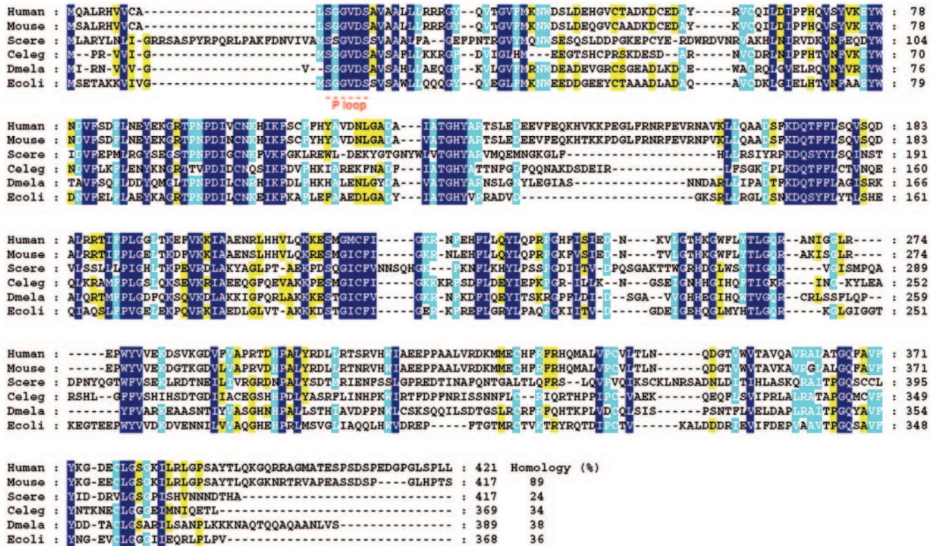
FIG. 1. Sequence alignment of mt tRNA-specific 2-thiouridylases. Human MTU1 (AB178028) was aligned with its mouse (AAH61026), yeast (Scere, CAA98591), C. elegans (Celeg, Q17440), D. melanogaster (Dmela, AAE45578), and E. coli counterparts (P25745). Multiple alignment of each sequence was performed by using ClustalW (62) and displayed using the Genedoc multiple sequence alignment editor. Homology values (between the human sequence and the others), as calculated by Genedoc (63), are shown at the end of the alignment. The colored boxes indicate the degree of sequence similarity. The P loop motif (12–17) is indicated by a dotted red line.
