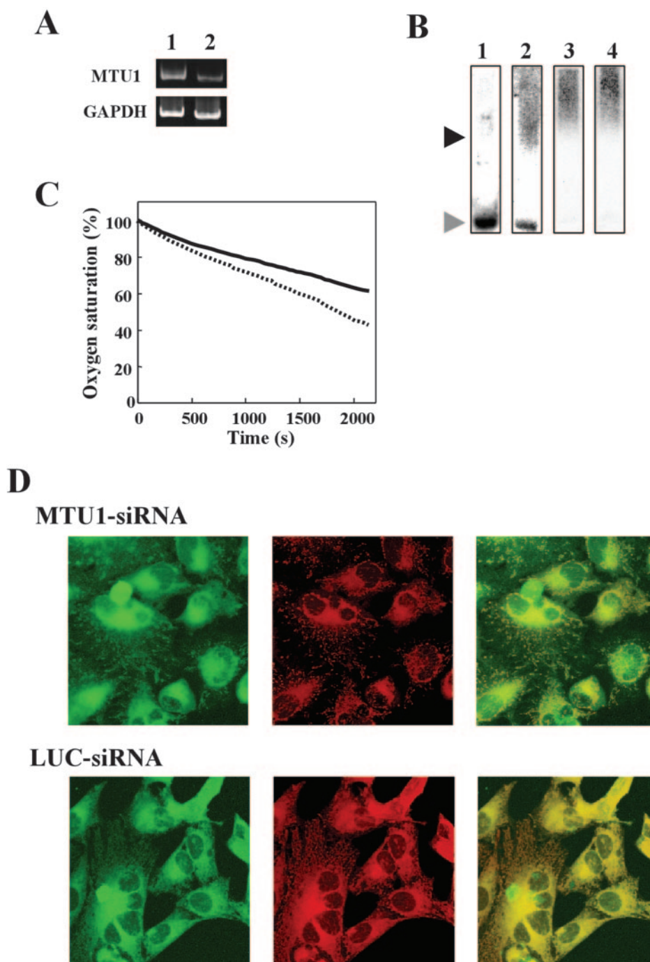
FIG. 6. siRNA-induced knockdown of human MTU1 results in mitochondrial dysfunction. A , the MTU1 mRNA levels of HeLa cells transfected with siRNAs that target MTU1 ( MTU1 -1) (lane 2) or luciferase (lane 1) were quantified by RT-PCR (35 cycles). Glyceraldehyde-3-phosphate dehydrogenase mRNA was quantified as a control. B , APM-Northern analysis of the 2-thiolation of mitochondrial (lanes 1 and 2) or cytosolic (lanes 3 and 4) tRNAs Lys molecules from HeLa cells transfected with siRNAs that target MTU1 (lanes 1 and 3) or luciferase (lanes 2 and 4). The retarded bands of the 2-thiolated tRNAs are marked by a black arrowhead. The non-retarded bands of non-thiolated tRNAs are marked by a gray arrowhead. C , the rates of oxygen consumption of HeLa cells transfected with siRNAs targeting MTU1 (dotted line) or luciferase (solid line) were measured by a Clark type electrode. D , visualizing the mitochondrial membrane potential of MTU1 -knocked down HeLa cells. The cells transfected with siRNAs targeting MTU1 or luciferase are shown in the upper and lower panels, respectively. The mitochondria were visualized by staining the cells with MitoTracker Green (left panels), and its membrane potentials were simultaneously indicated by staining with MitoTracker Red (middle panels). Both panels were merged (right panels) to show the different intensities of the two fluorescence patterns.
