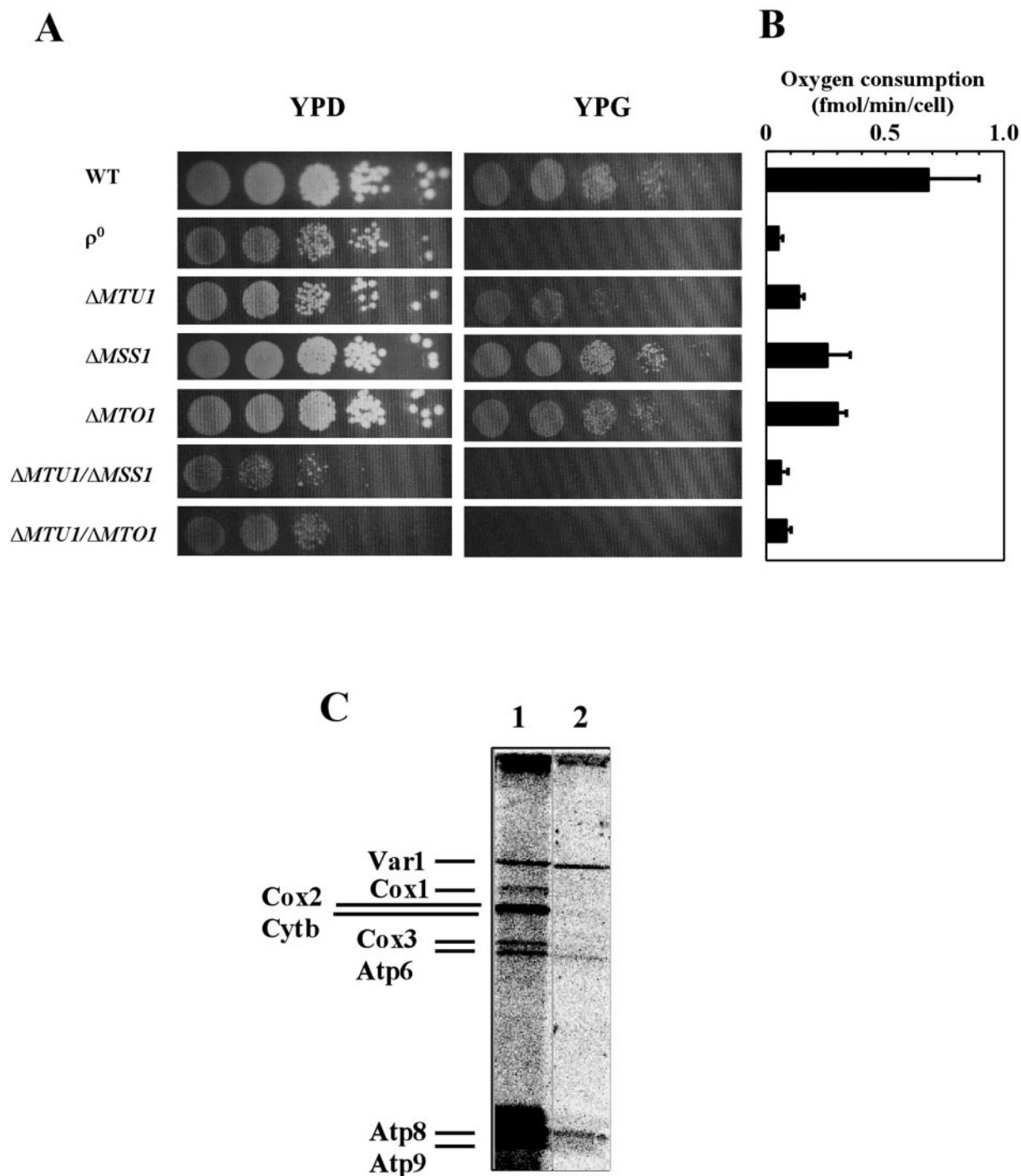
FIG. 4. Growth properties and mitochondrial activity of strains lacking the enzymes that modify the wobble position of mt tRNAs. A, growth of the wild type, three single deletion mutant ( \Delta MTU1 , \Delta MTO1 , and \Delta MSS1 ) and two double deletion mutant ( \Delta MTU1/\Delta MSS1 and \Delta MTU1/\Delta MTO1 ) strains. Each strain was serially diluted starting with 10^5 cells and then spotted onto fermentable YPD and non-fermentable YPG plates and incubated at 30 °C for 72 h. B, oxygen consumption of each mutant strain. The rate of oxygen consumption is shown along with the S.D. values obtained from three independent experiments. C, mitochondrial protein synthesis in the wild type (lane 1) and \Delta MTU1 (lane 2) strains was determined by in vivo pulse-labeling of mt DNA products with [ ^{35} S]methionine. The mt DNA products are identified on the left.
