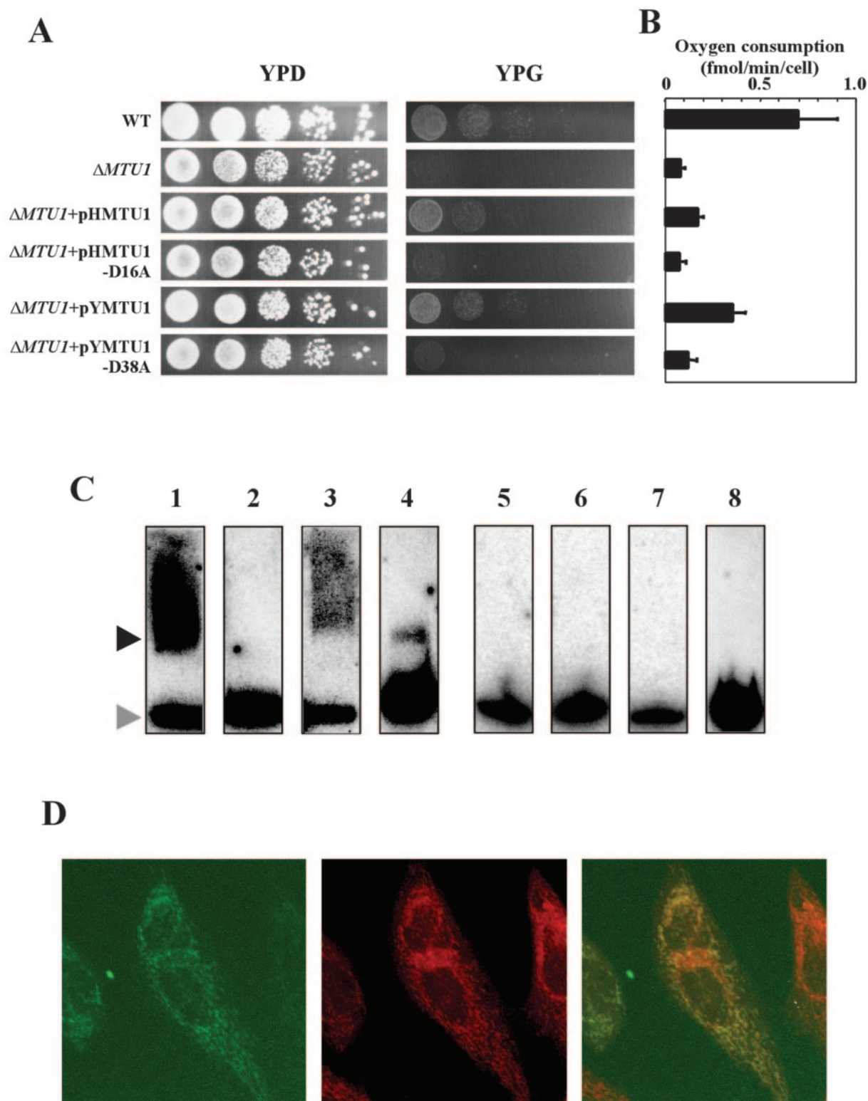
FIG. 5. Suppression of the respiratory defect of \Delta MTU1 by introducing the human or yeast MTU1 genes and mitochondrial localization of the MTU1 protein. A , growth of the wild type, \Delta MTU1 , and the MTU1 strain bearing a plasmid encoding the yeast MTU1 (pYMTU1) or human MTU1 (pHMTU1) gene. Also examined were MTU1 strains bearing pYMTU1 or pHMTU1 containing an inactivating mutation (pYMTU1-D38A and pHMTU1-D16A, respectively). Starting with 10^5 cells, serial dilutions were spotted onto YPD, and YPG plates and incubated at 30 °C for 72 h. B , rate of oxygen consumption for each strain. The rate of oxygen consumption is shown along with the S.D. values obtained from three independent experiments. C , APM-Northern analysis of the 2-thiolation in the mt tRNA Lys molecules from the wild type (lanes 1 and 5), \Delta MTU1 (lanes 2 and 6), \Delta MTU1 with pYMTU1 (lanes 3 and 7), and \Delta MTU1 with pHMTU1 (lanes 4 and 8) strains. The polyacrylamide gels of lanes 1–4 contain APM, while the gels of lanes 5–8 lack APM. The retarded bands of the 2-thiolated tRNAs are marked by a black arrowhead. The non-retarded bands of the non-thiolated tRNA are marked by a gray arrowhead. D , mitochondrial localization of the MTU1 protein. HeLa cells were transiently transfected with pHMTU1/EGFP, which expresses human MTU1 fused with EGFP. The intracellular localization of the MTU1 -EGFP fusion protein was then visualized by the green fluorescence of EGFP by using a confocal fluorescence microscope (left panel). The mitochondria were stained by MitoTracker Red (Molecular Probes), and its red fluorescence was simultaneously observed (middle panel). Both panels were merged (right panel) to show the complete overlap of the two fluorescence patterns.
