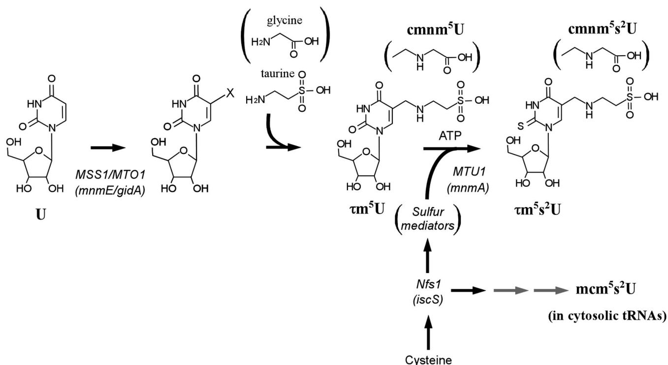
FIG. 7. Biosynthetic pathway that introduces the \gamma\text{m}^5\text{s}^2\text{U} ( \text{cmnm}^5\text{s}^2\text{U} ) modification of mitochondrial tRNAs. MSS1 and MTO1 are involved in the initial step of \gamma\text{m}^5\text{s}^2\text{U} ( \text{cmnm}^5\text{s}^2\text{U} ) synthesis on mt tRNAs. Mitochondrial taurine or glycine is subsequently incorporated into mt tRNAs by unidentified transferases to build \gamma\text{m}^5\text{s}^2\text{U} or \text{cmnm}^5\text{s}^2\text{U} , respectively. Nfs1 is responsible for the initial step in the 2-thiolation of \gamma\text{m}^5\text{s}^2\text{U} ( \text{cmnm}^5\text{s}^2\text{U} ) in mt tRNAs and \text{mcm}^5\text{s}^2\text{U} in cytoplasmic tRNAs (20). The sulfur from cysteine is transferred to unknown sulfur mediators by Nfs1p . MTU1 then acts as a mitochondria-specific 2-thiouridylase for \gamma\text{m}^5\text{s}^2\text{U} ( \text{cmnm}^5\text{s}^2\text{U} ) by using the activated sulfur from the mediators.
