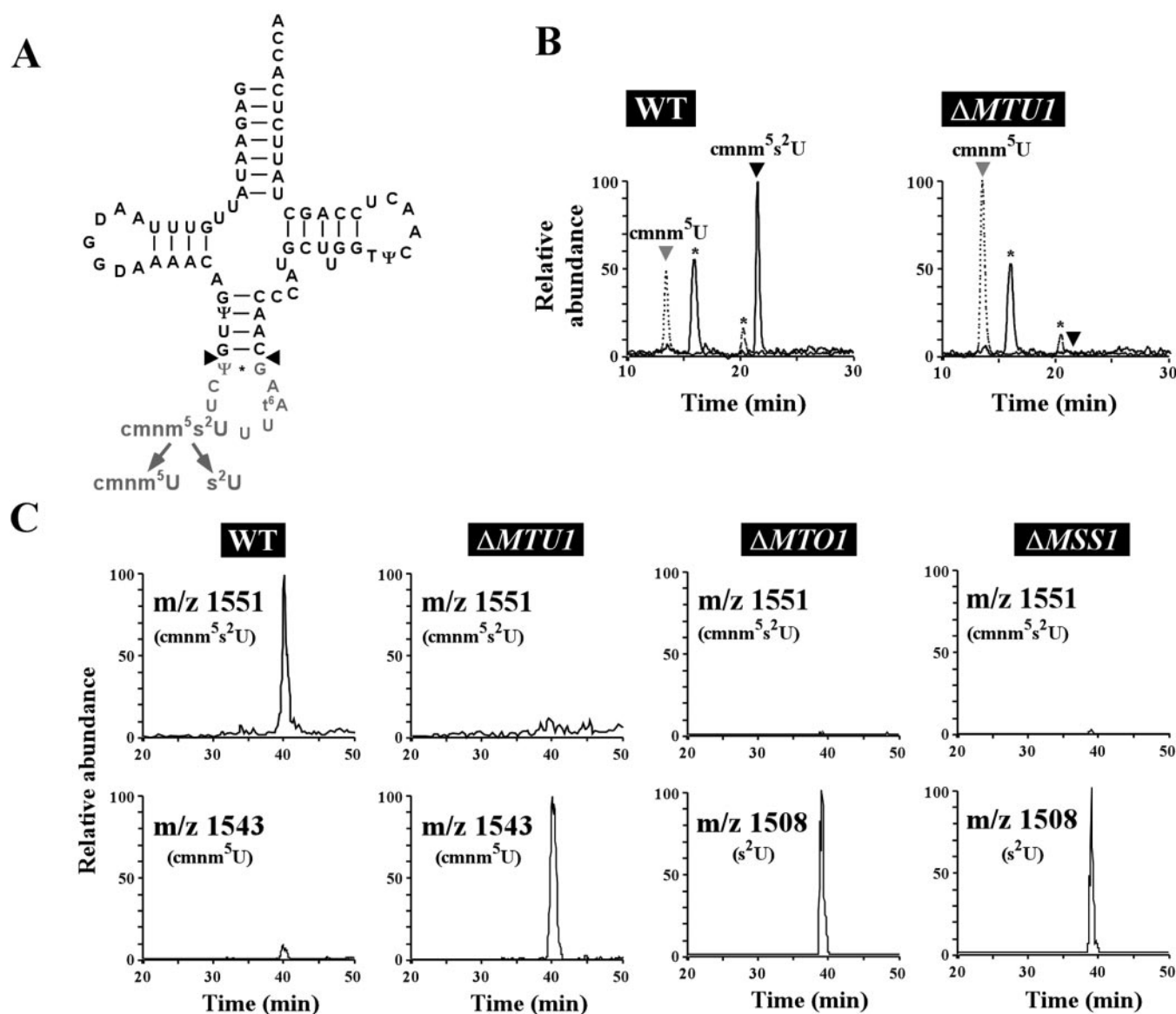
FIG. 3. Mass spectrometric analysis of the tRNAs from the wild type and \Delta MTU1 yeast strains. A , the secondary structure of yeast mt tRNA Lys bearing the following post-transcriptional modifications: dihydrouridine ( D ), pseudouridine ( \Psi ), ribothymidine ( T ), N 6 -threonylcarbamoyl-adenosine ( t 6 A ), 5-carboxymethylaminomethyl-2-thiouridine ( cmnm 5 s 2 U ), 5-carboxymethylaminomethyluridine ( cmnm 5 U ), and 2-thiouridine ( s 2 U ). The anticodon-containing fragment produced by digesting the tRNA with RNase T 1 is colored gray. The cleavage positions are shown by arrowheads. B , LC/MS analysis of the total nucleosides in the mt tRNA Lys molecules obtained from the wild type ( left panel ) and \Delta MTU1 ( right panel ) strains. Mass chromatograms of cmnm 5 U ( m/z 332 at retention time 13.4, dotted line ) and cmnm 5 s 2 U ( m/z 348 at RT 21.6, solid line ) are shown by the proton adduct form of each nucleoside. Side peaks in RT 15.9 and RT 20.3 ( asterisks ) are assigned as artifacts with unknown chemical structures. C , LC/MS fragment analysis of RNase T 1 -digested mt tRNA Lys molecules obtained from the wild type, \Delta MTU1 , \Delta MTO1 , and \Delta MSS1 strains. The mass chromatogram of doubly charged ions in the anticodon-containing fragment bearing cmnm 5 s 2 U ( m/z 1551) is shown in each of the upper panels . Mass chromatograms of the same fragments bearing cmnm 5 U ( m/z 1543) are shown in the lower left panels for wild type and \Delta MTU1 , whereas the mass chromatograms of the same fragments carrying s 2 U ( m/z 1508) are shown in the lower right panels for \Delta MTO1 and \Delta MSS1 .
