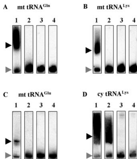
FIG. 2. APM gel electrophoresis combined with Northern blotting of yeast mitochondrial tRNAs. The presence of 2-thio modifications of the mt tRNA Gln (A), mt tRNA Lys (B), mt tRNA Glu (C), and cytoplasmic tRNA Lys (D) molecules in wild type yeast (lanes 1 and 3) or \Delta MTU1 yeast (lanes 2 and 4) were analyzed by APM gel electrophoresis and Northern blotting. The gels of lanes 1 and 2 contain APM, whereas the gels of lanes 3 and 4 lack APM. The retarded bands of the 2-thiolated tRNAs are marked by a black arrowhead, whereas the non-retarded bands of the unthiolated tRNAs are marked by a gray arrowhead.
