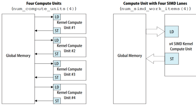
Fig. 2: Multiple parallel CU (left) versus single CU with SIMD (right).
